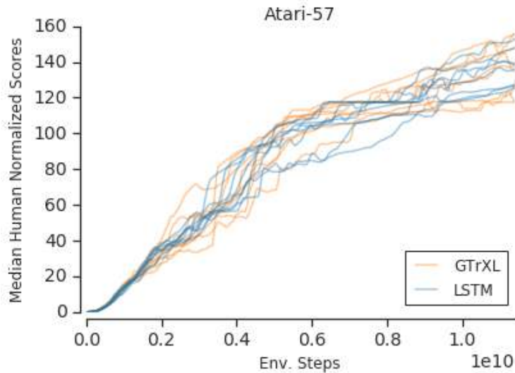
Figure 11: Median human-normalized returns as training progresses for both GTrXL and LSTM models. We run 8 hyperparameter settings per model.
