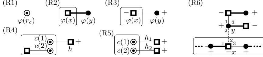
Fig. 6. Figure (R i ) shows a subgraph of G^\delta illustrating Extension Rule i , for i \in \{1, 2, \dots, 6\} . We represent agents of \varphi(X) by enclosing them in a rectangular box. Bold edges represent \bar{E}_{M_0} and normal edges represent \bar{E}_M .
