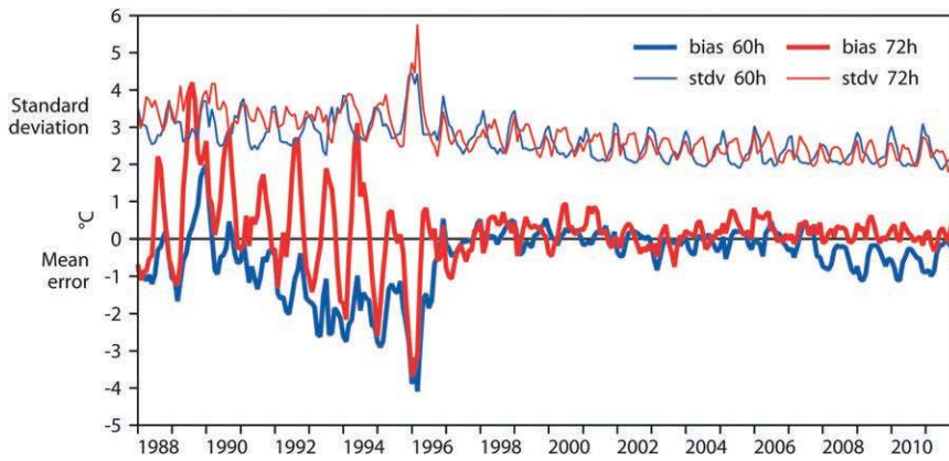
FIG. 1. Long-term history of 2-m temperature errors ( ^{\circ}\text{C} ) of daily 60-h (blue, verifying at 0000 UTC) and 72-h forecasts (red, verifying at 1200 UTC) in the ECMWF model over Europe. Mean errors are given with thick solid lines and standard deviations with thin lines on basis of monthly averages of model errors with respect to about 700 SYNOP stations over Europe.
