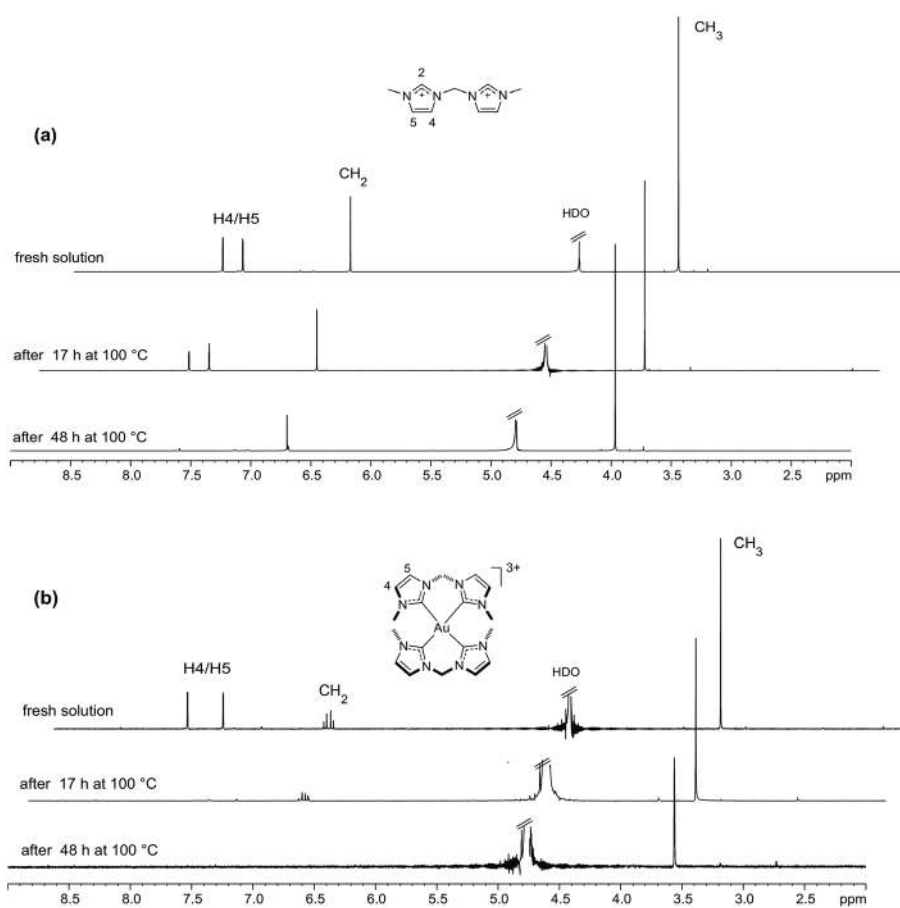
Fig. 7 ^1\text{H} NMR spectra (600.13 MHz, \text{D}_2\text{O} ) for solutions of (a) the imidazolium salt \text{L}^1\text{-}2\text{HCl} and (b) the \text{Au}^{\text{III}} complex [\text{Au}(\text{L}^1)_2]^{3+} (prepared from [\text{Au}(\text{L}^1)_2\text{Cl}_2]\text{Cl} 2 ), showing disappearance of signals due to H/D exchange reactions. For \text{L}^1\text{-}2\text{HCl} , no signal for the H2 protons was detected even from freshly-prepared solutions.
