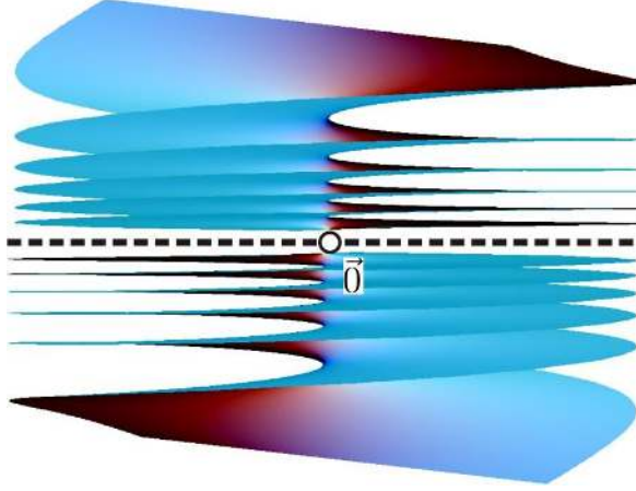
Figure 15: The origin is a singular leaf point of the horizontal disk passing through it, but not of the two non-proper spiraling leaves L^+, L^- .
