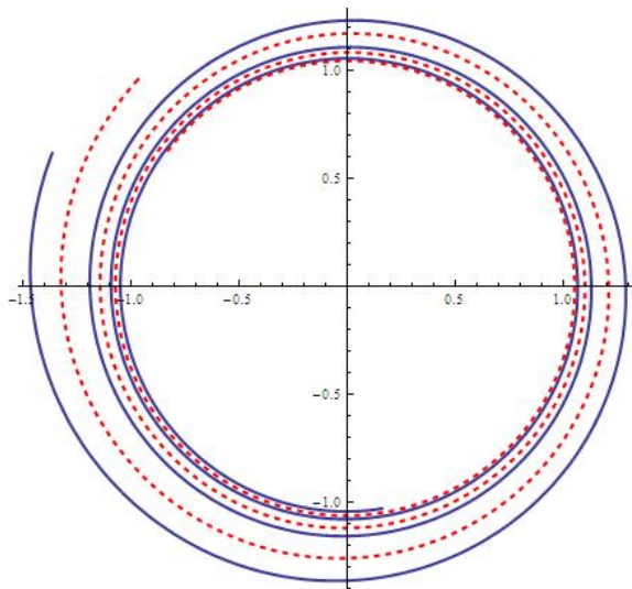
Figure 4: A lamination consisting of three leaves: \mathbb{S}^1 and two disjoint spirals which limit to \mathbb{S}^1 .
