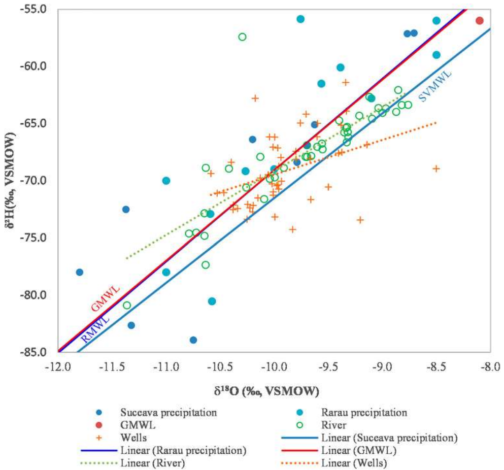
Figure 3. Local Meteoric Water Lines and River Water Lines for precipitation (blue line), surface (green line) and groundwaters (orange line) in the Suceava Watershed.
