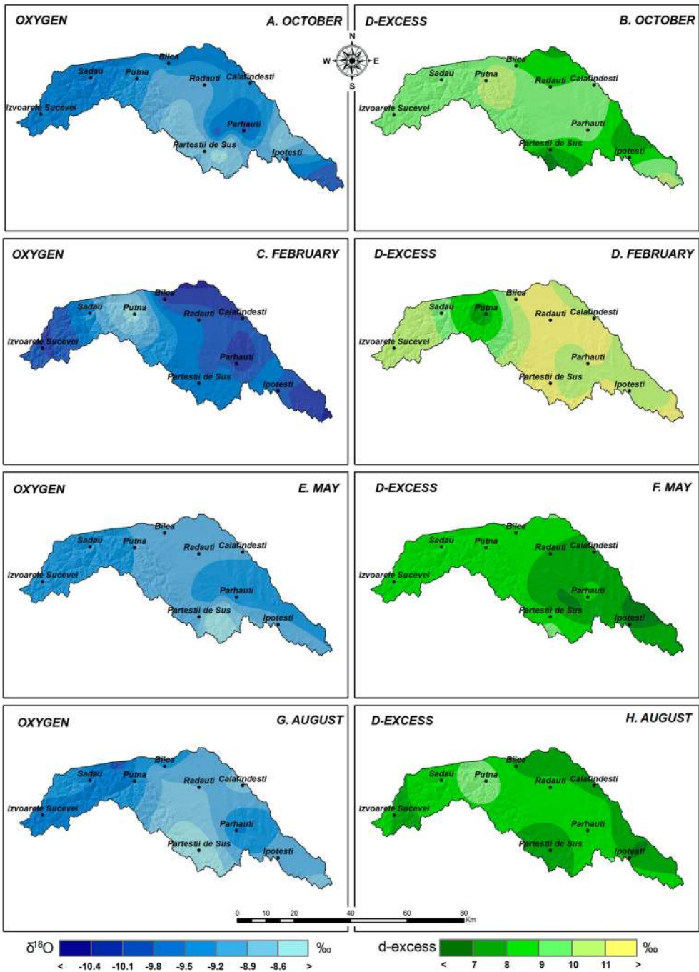
Figure 8. Seasonal distribution of \delta^{18}\text{O} (left panel) and d -excess (right panel) in groundwater in the Suceava River watershed based on empirical semivariogram [51,52].
