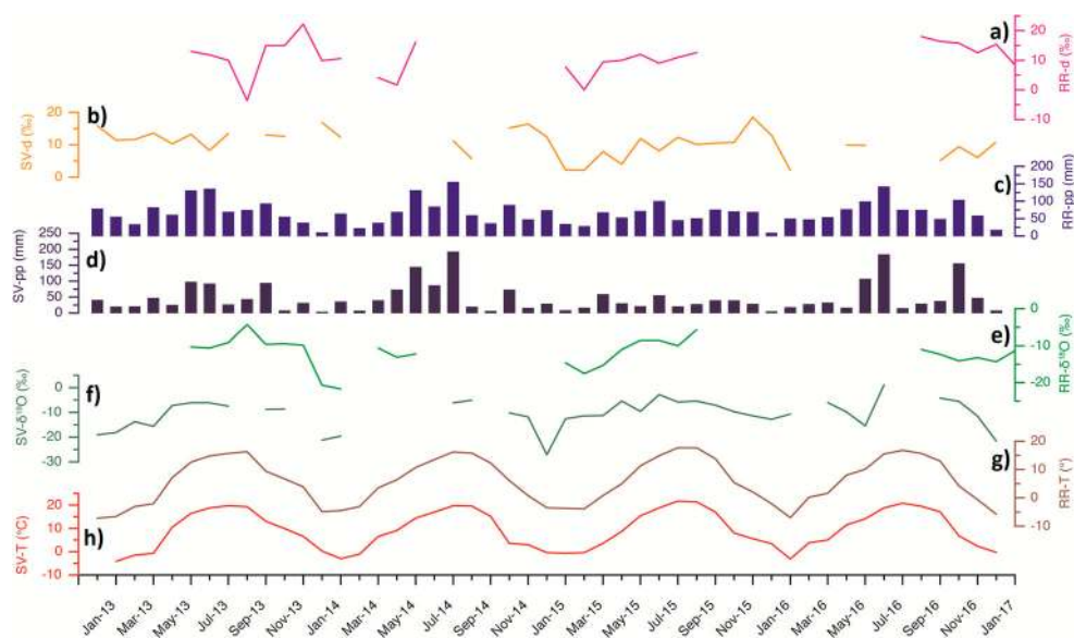
Figure 2. Monthly time series d -excess (d) at (a) Rarău station (RR) and (b) Suceava station (SV), precipitation amount (pp) at RR (c) and SV (d), precipitation ( \delta^{18}\text{O} ) at RR (e) and SV (f) and air temperature (T) at RR (g) and SV (h).
