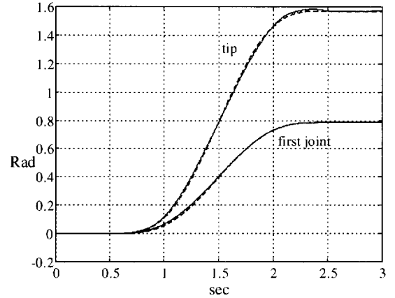
Figure 2: Desired (dashed) and actual trajectories
