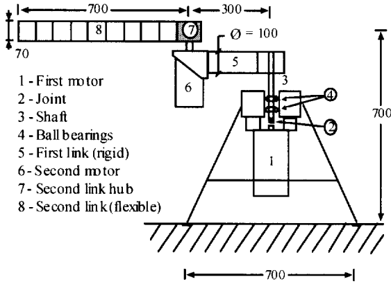
Figure 1: The FLEXARM
