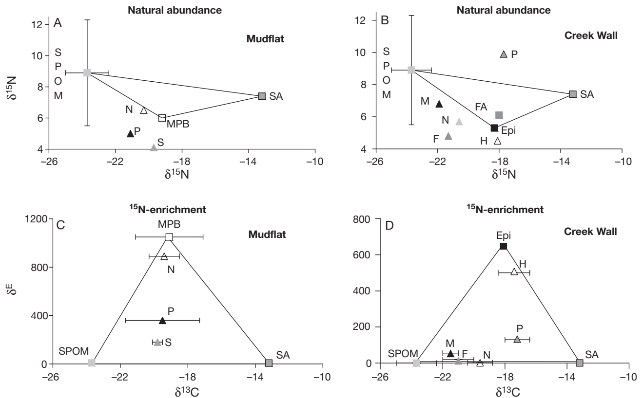
Fig. 2. Natural abundance stable isotope values ( \delta^{15}\text{N} and \delta^{13}\text{C} ; prior to isotope additions) for (A) mudflat and (B) creek wall; and ^{15}\text{N} -enrichment ( \delta^E , highest) in primary producers and infauna during the 21 d experiment plotted against an average \delta^{13}\text{C} found over the 21 d experiment in (C) mudflat and (D) creek-wall habitats. Isotope values are corrected for trophic enrichment (see 'Materials and methods—Mixing models and trophic enrichment factors'). Primary producers are squares; infauna are triangles. The polygons connect the 3 sources used in the mixing model. SPOM: suspended particulate organic matter, MPB: microphytobenthos, FA: filamentous algae, Epi: epiphytes, N: Nereis diversicolor , S: Streblospio benedicti , P in mudflat: Paranais litoralis , P in creek wall: Pygospio elegans , M: Manayunkia aestuarina , F: Fabricia sabella , H: Heterolaophonte sp. Consumers with values outside the mixing triangles were assumed to fall on the nearest mixing line, a possibility consistent with isotope variation in the source (apex) plant isotope values
