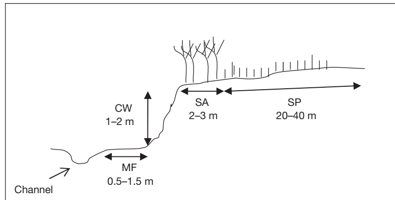
Fig. 1. Modified schematic (not to scale) from Johnson et al. (2007) of sampled saltmarsh habitats with approximate size ranges of habitats: mudflat (MF), creek wall (CW), Spartina alterniflora understory (SA) and S. patens understory (SP)
