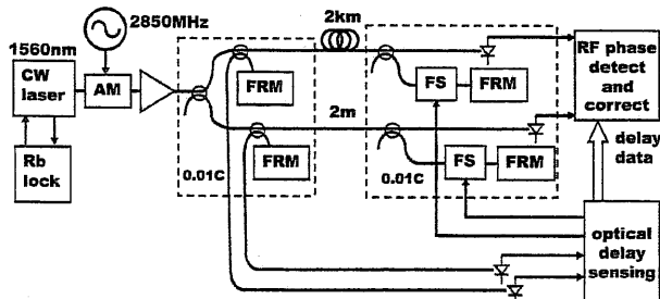
Fig. 2. Dual-channel transmission experiment. The frequency is 2850 MHz.
