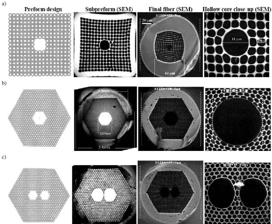
Fig. 17. Hollow core PBG fibers: a) square lattice single core (fiber diameter 125 \mu\text{m} , lattice constant 3.6 \mu\text{m} , d/\Lambda = 0.94 , core diameter 11 \mu\text{m} ); b) hexagonal lattice single core (fiber diameter 130 \mu\text{m} , lattice constant 3 \mu\text{m} , d/\Lambda = 0.93 , core diameter 31 \mu\text{m} ); c) hexagonal lattice double core (fiber diameter 117 \mu\text{m} , lattice constant 2.9 \mu\text{m} , d/\Lambda = 0.93 , diameter of each core 18 \mu\text{m} )
