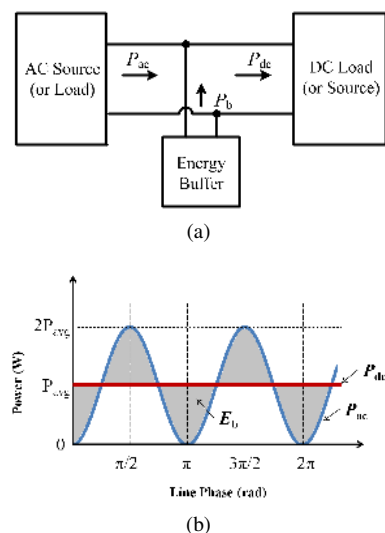
Fig. 1. Mismatch in instantaneous power between single-phase ac, P_{ac} , and constant power dc, P_{dc} , results in the need for an energy buffer, as shown in (a), to absorb and supply the energy, E_b , indicated by the shaded area in (b).
