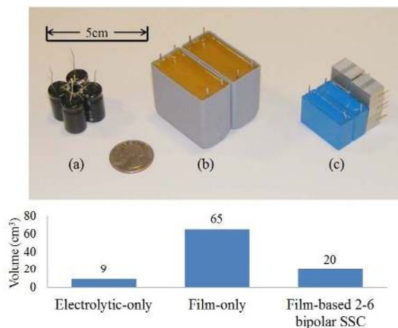
Fig. 20. Relative size of passive energy storage components in different energy buffer architectures: (a) electrolytic-capacitor-only ( 9 \text{ cm}^3 ) (b) film-capacitor-only ( 65 \text{ cm}^3 ) and (c) film-capacitor-based SSC ( 20 \text{ cm}^3 ) energy buffer.
