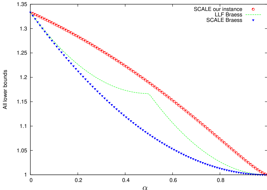
Figure 4: The performance of the SCALE policy on our hard instance from Section 3 vs. the performance of the LLF and SCALE policies on the instance of the Braess paradox. Observe that SCALE outperforms LLF on the latter instance.
