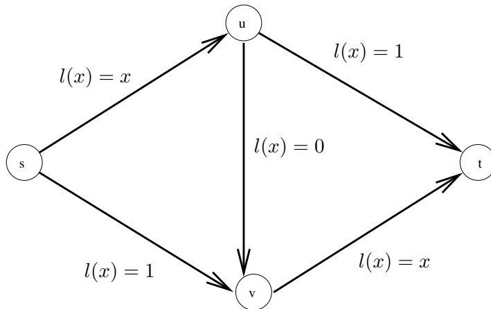
Figure 1: The Braess paradox instance.
