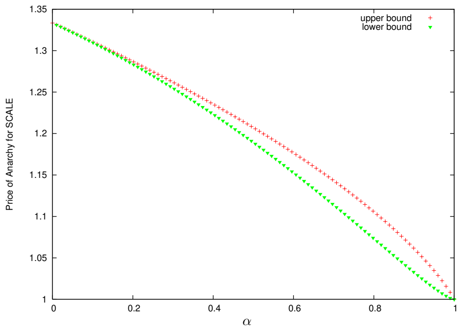
Figure 2: Our upper and lower bounds for SCALE, as obtained in Section 3 plotted as functions of the fraction \alpha of the users that are coordinated.
