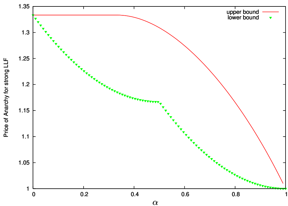
Figure 3: Our upper bound for strong LLF, as obtained in Section 3, under the further assumption that \lambda = \alpha . The lower bound is the exact performance of LLF on the instance of the Braess paradox.
