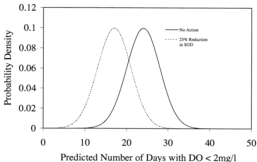
Figure 3. Conditional risk profiles for number of hypoxic days. The dashed line shows the conditional distribution for hypoxic days assuming a reduction in sediment oxygen demand of 25%. The solid line represents the base-case scenario.
