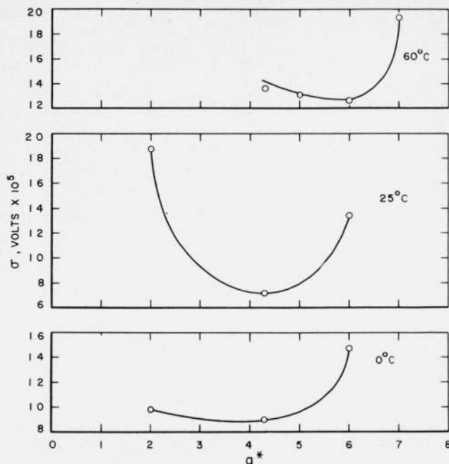
FIGURE 1. Standard deviation of E^{o'} from the least-square line as a function of a^* at 0°, 25°, and 60° C.
