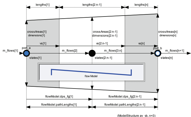
Figure 3: Overview of PartialTwoPortFlow
