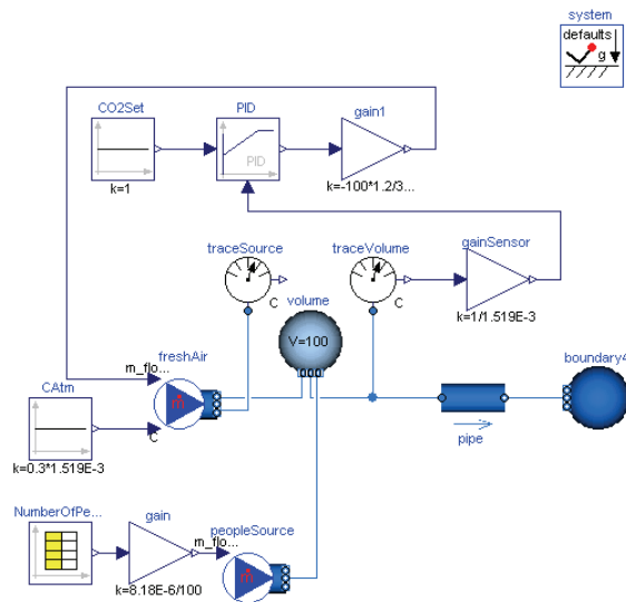
Figure 12: Example model for trace substances.
