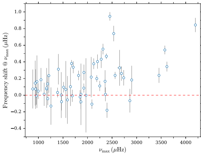
Figure 2. Frequency shift at \nu_{\max} from line-of-sight velocities of the stars in the sample (see Table 1). The uncertainty indicates for a given target the minimum frequency uncertainty of the five radial modes nearest \nu_{\max} . The frequency uncertainty on individual modes is in several cases lower than the line-of-sight frequency shift. Large or small, the systematic shift can thus cause bias in the modeling if left uncorrected.
