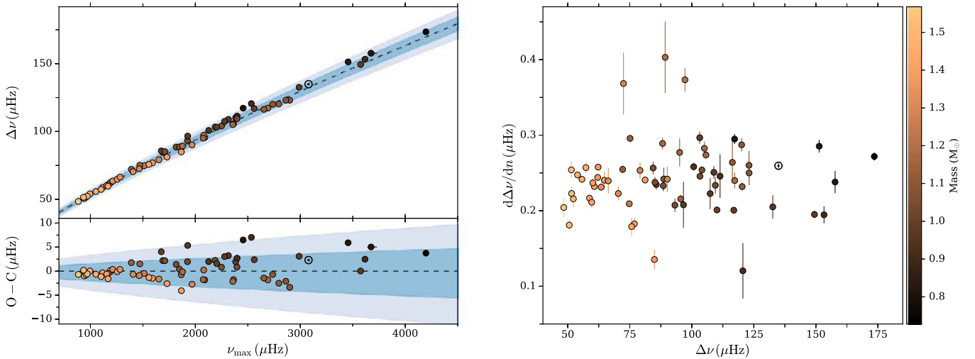
Figure 9. Left: measured values of \Delta\nu against \nu_{\max} from fitting of Equation (27), with the color indicating the modeled mass. The dashed line shows the empirical relation by Huber et al. (2011), with the 1 and 2\sigma uncertainties on the relation given by the dark and light blue regions. From our values we calculate a correlation of \rho_{\alpha,\beta} = -0.99913 between the \alpha and \beta parameters of the Huber et al. (2011) relation—this was included to estimate the uncertainty regions. The bottom panel shows the residuals of the measured values to the relation. Measured values are seen to overall agree well with expectations, with a modest mass gradient across the residuals. Right: measured gradient of \Delta\nu with radial order, d\Delta\nu/dn , defining the overall curvature of the ridges in the échelle diagram against \Delta\nu .
