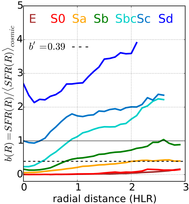
Fig. 9. Radial profiles of the birthrate parameter, b(R) , averaged in seven Hubble type bins; b(R) compares the present to the past-average SFR at radius R (cf. Eq. (4)). The dashed and solid black lines indicate our (volume-corrected) value for the local Universe and the reference value b(R) = 1 , respectively.
