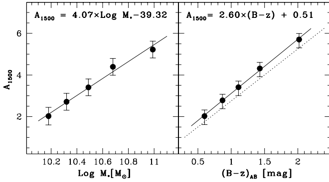
Figure 5. Left: UV light attenuation ( A_{1500} = 2.5 \times \text{Log}(\text{SFR}_{1.4 \text{ GHz}}/\text{SFR}_{1500}) ) as a function of galaxy stellar mass. Right: UV light attenuation as a function of B-z color (UV slope). The dotted line shows the attenuation law derived in Daddi et al. (2004) as described in the text.
