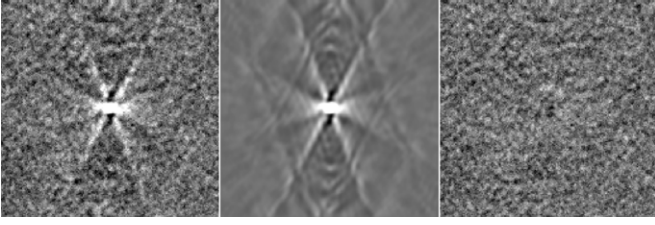
Figure 2. Left: median stacking result of all the 34000 sBzK galaxies. Middle: best-fit dirty beam convolved Gaussian to the stacked data. The total flux recovered is 8.8 \pm 0.1 \mu\text{Jy} . Right: residual image.
