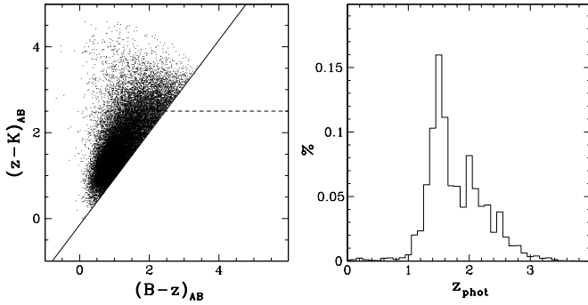
Figure 1. Left: the selection diagram for sBzK star-forming galaxies at z \approx 2 . Right: photometric redshift distribution of the COSMOS sBzK sample. The bulk of the sample spans the redshift range [1.3–2.5].
