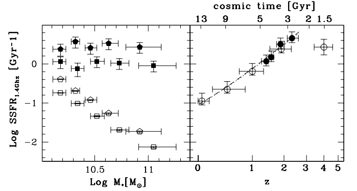
Figure 4. Left: radio derived SSFR (solid symbols) at z \approx 1.6 (squares) and \approx 2.1 (pentagons) are compared to the uncorrected UV derived SSFR (empty symbols) as a function of \text{Log } M_* . Right: radio derived SSFRs from this work (solid dots), for star-forming galaxies with M_* \sim 3 \times 10^{10} M_{\odot} , as a function of redshift at z \approx 1.4, 1.6, 1.9, 2.3 . Literature data are plotted as empty circles. The dotted curve shows the SSFR as a function of redshift described by Equation (2).
