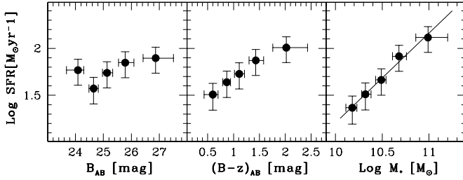
Figure 3. Total radio-derived SFR vs. B band (left), B-z color (middle), and stellar mass (right). The solid line is the best-fit line: \text{Log}(\text{SFR}) \propto 0.95 \text{Log } M_* .
