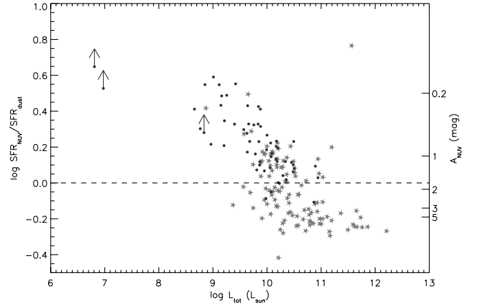
FIG. 5.—Plot of \log(\text{SFR}_{\text{NUV}}/\text{SFR}_{\text{dust}}) vs. \log L_{\text{tot}} . Symbols are as in Fig. 3. The right y-axis indicates the NUV dust attenuation. [See the electronic edition of the Supplement for a color version of this figure.]
