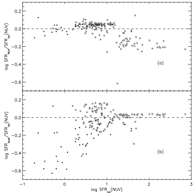
FIG. 7.—(a) Plot of \log[SFR_{\text{NUV}}/SFR_{\text{tot}}(\text{NUV})] vs. \log SFR_{\text{tot}}(\text{NUV}) . (b) Plot of \log[SFR_{\text{dust}}/SFR_{\text{tot}}(\text{NUV})] vs. \log SFR_{\text{tot}}(\text{NUV}) . Symbols are as in Fig. 3. [See the electronic edition of the Supplement for a color version of this figure.]
