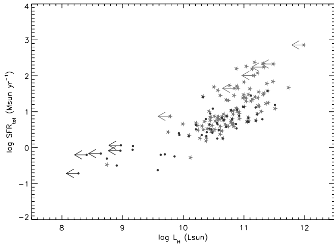
FIG. 11.— H -band luminosity vs. SFR_{\text{tot}} . Symbols are as in Fig. 3. [See the electronic edition of the Supplement for a color version of this figure.]
