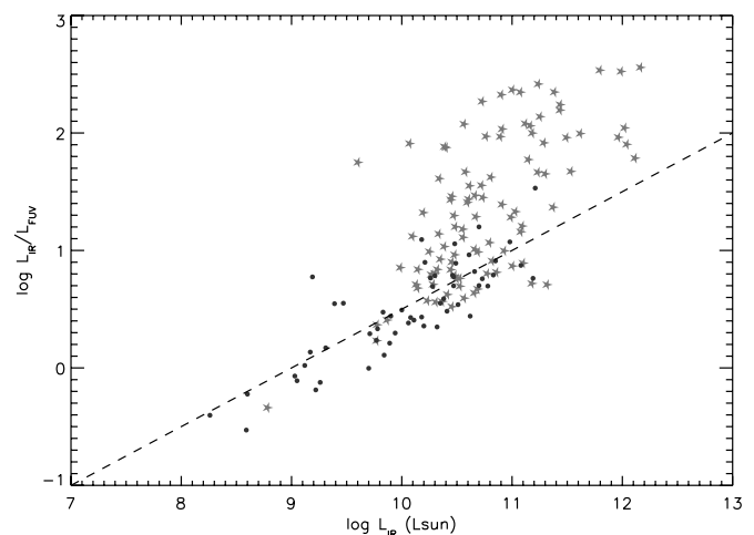
FIG. 8.—Plot of L_{\text{IR}} vs. L_{\text{IR}}/L_{\text{FUV}} . Symbols are as in Fig. 3. The dashed line corresponds to the relation L_{\text{IR}}/L_{\text{FUV}} \sim (L_{\text{IR}}/10^9)^{1/2} of Bell (2003). [See the electronic edition of the Supplement for a color version of this figure.]
