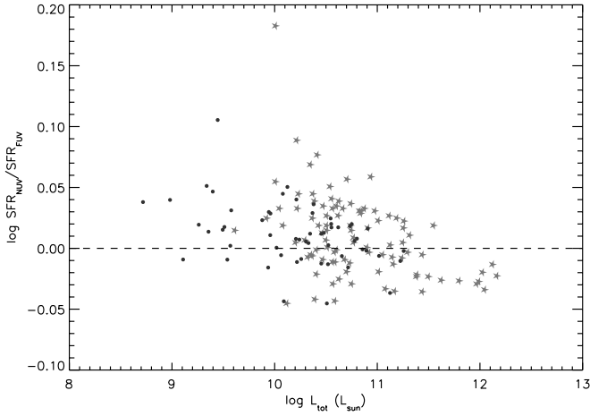
FIG. 4.—Plot of \log(\text{SFR}_{\text{NUV}}/\text{SFR}_{\text{FUV}}) vs. \log L_{\text{tot}} . Symbols are as in Fig. 3. [See the electronic edition of the Supplement for a color version of this figure.]
