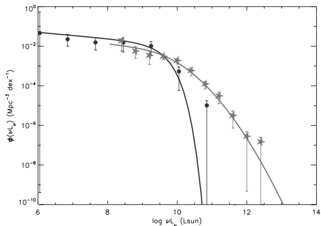
FIG. 1.—NUV (circles) and 60 \mu\text{m} (stars) LFs for the NUV- and FIR-selected samples. The lines connecting the circles and stars correspond to the NUV and 60 \mu\text{m} LFs from Wyder et al. (2005) and Takeuchi et al. (2003) respectively. Error bars correspond to 1 \sigma uncertainty. [See the electronic edition of the Supplement for a color version of this figure.]
