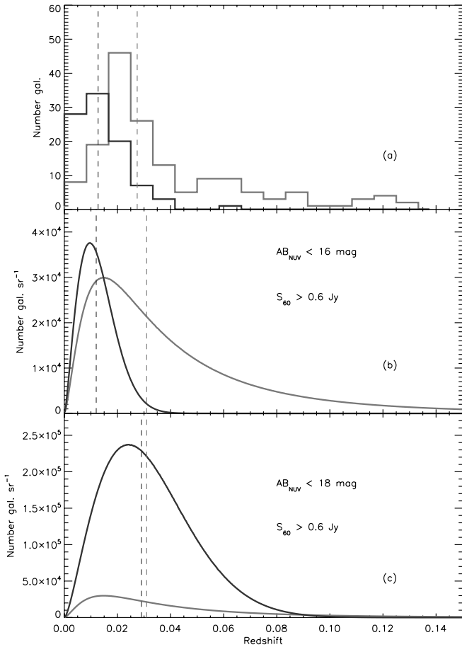
FIG. 2.—(a) Redshift distributions for the NUV (darker histogram) and FIR (lighter histogram) selected galaxies. (b) Theoretical redshift distributions for samples of galaxies with the same limiting fluxes as our samples. (c) Same as (b), but for an NUV-selected sample with AB_{\text{NUV}} \leq 18 mag. Vertical dashed lines in the three panels correspond to the median values of each distribution. [See the electronic edition of the Supplement for a color version of this figure.]
