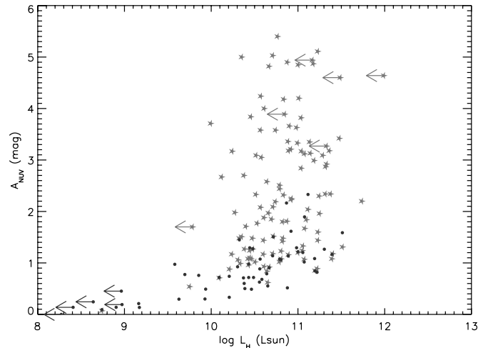
FIG. 12.— H -band luminosity vs. A_{\text{NUV}} . Symbols are as in Fig. 3. [See the electronic edition of the Supplement for a color version of this figure.]
