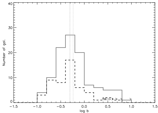
FIG. 9.—Distribution of \log b for the NUV ( dashed histogram ) and the FIR ( solid histogram ) selected samples. The vertical dotted lines correspond to the median values of the distributions. Arrows correspond to nominal limiting values. [See the electronic edition of the Supplement for a color version of this figure.]
