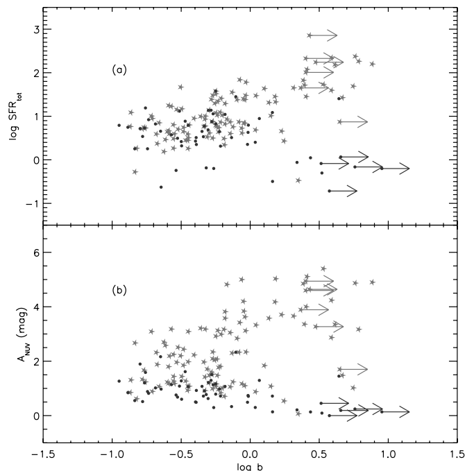
FIG. 10.—(a) Plot of \text{SFR}_{\text{tot}} vs. b . (b) Plot of A_{\text{NUV}} vs. b . Symbols are as in Fig. 3. [See the electronic edition of the Supplement for a color version of this figure.]
