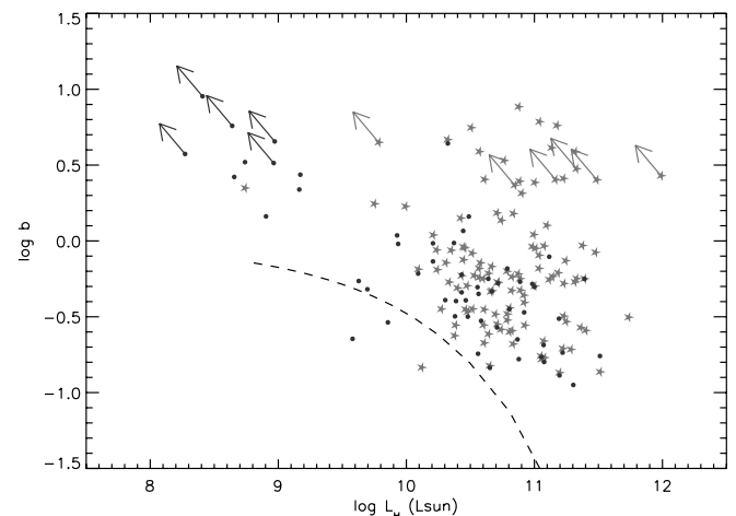
FIG. 13.— H -band luminosity vs. b . Symbols are as in Fig. 3. The dashed line corresponds to the calibration of Boselli et al. (2001) for their sample of late-type galaxies from nearby clusters with a normal H I content. [See the electronic edition of the Supplement for a color version of this figure.]
