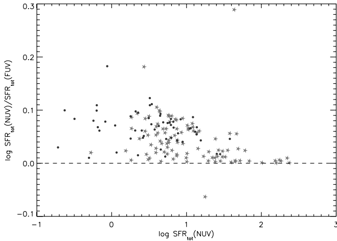
FIG. 6.—Plot of \log [SFR_{\text{tot}}(\text{NUV})/SFR_{\text{tot}}(\text{FUV})] vs. \log SFR_{\text{tot}}(\text{NUV}) . Symbols are as in Fig. 3. [See the electronic edition of the Supplement for a color version of this figure.]
