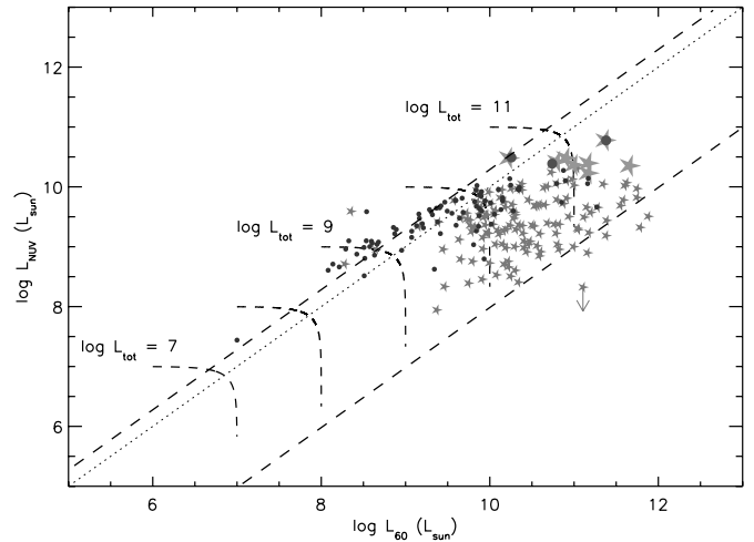
FIG. 3.—Plot of L_{60} vs. L_{\text{NUV}} (not corrected for attenuation) for the NUV (circles) and FIR (stars) selected samples. Arrows indicate upper limits. Dashed curves represent the loci of points with L_{\text{tot}} = 10^7, 10^8, 10^9, 10^{10}, and 10^{11} L_{\odot} , respectively. The dotted line corresponds to L_{\text{NUV}} = L_{60} . The lower dashed line corresponds to the maximum attenuation below which the FIR-selected sample is complete, and the upper dashed line corresponds to the minimum attenuation above which the NUV-selected sample is complete. The larger stars and circles correspond to the UVLGs of the FIR- and NUV-selected samples, respectively. [See the electronic edition of the Supplement for a color version of this figure.]
