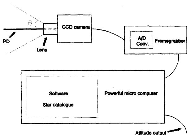
Fig. 1. Principle Diagram of a Second Generation Star Tracker. The Analog CCD Signal is Converted to a Digital Image in the Framegrabber. The Digital Image is Transformed into the Attitude Information by the Computer.
