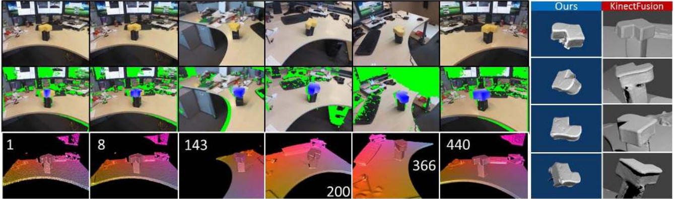
Figure 9. Film strip showing a comparison between our method and KinectFusion for 3D reconstruction. Each column shows a frame, the first row shows the color frame, the second row visualized our reconstruction result on re-projected color image (aligned with depth image), the third row shows the KinectFusion fusion frame. Last two columns shows the final reconstruction result of both methods.
