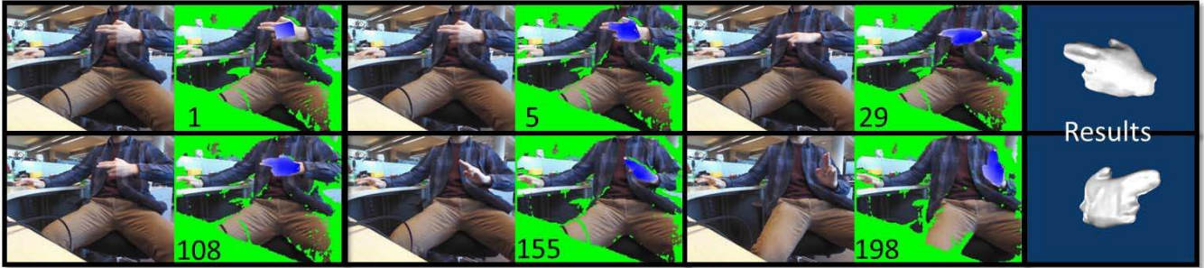
Figure 5. Film strip showing our algorithm tracking and reconstructing a hand with fixed articulation pose. For each frame, left shows the color image while right shows the reconstruction result overlaid with the color image reprojected onto the depth image. Green indicates missing depth data.
