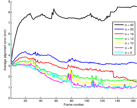
Figure 8. Quantitative evaluation of the accuracy of our method for 3D reconstruction with different \sigma .
