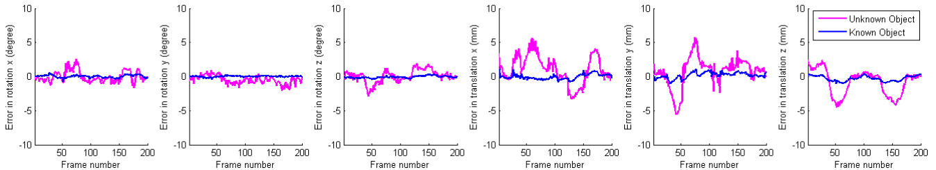
Figure 7. Quantitative evaluation of the precision our method for tracking 3D rigid object on synthetic data. The error in translation is measured in mm while rotation is measured in degree.
