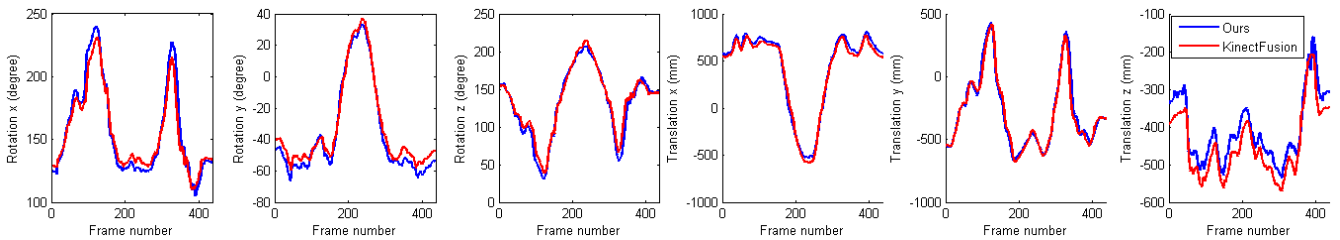
Figure 10. Quantitative comparison between camera pose output when using KinectFusion[7] and our method. Translation is measured in mm while rotation is measured in degree.
