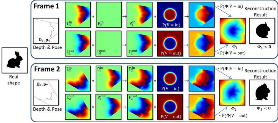
Figure 2. Work flow of our reconstruction framework.
