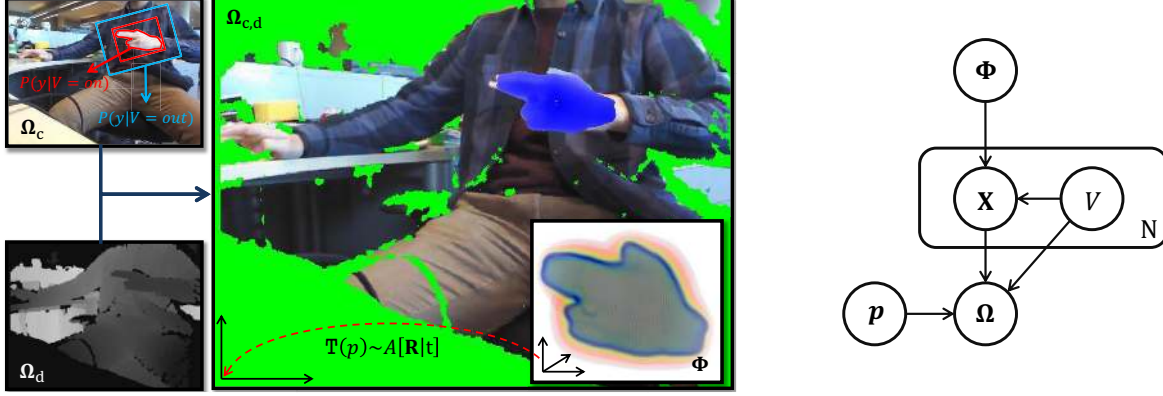
Figure 1. (Left): Representation of the 3D model \Phi , the RGB-D image domain \Omega_{c,d} , the surface / background models P(y|V = on) / P(y|V = out) and the pose T(\mathbf{p}) . (Right): Graphical model of our generative model for tracking and reconstruction.
