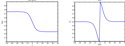
Figure 3. Plot of \mathcal{H}(z) (left) and L^{in} (right)
