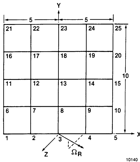
Figure 11. Square cantilever plate.
