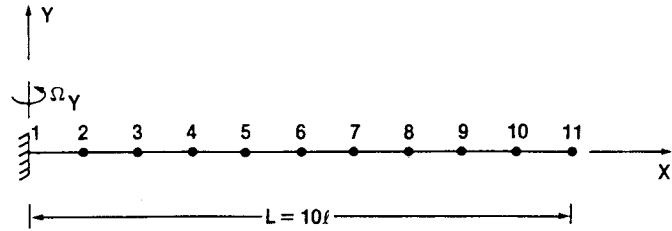
Figure 14. Spinning cantilever beam.
