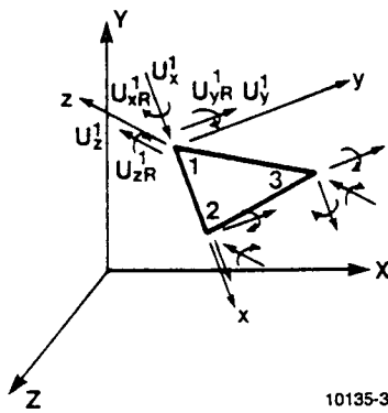
(c) Triangular shell element.
