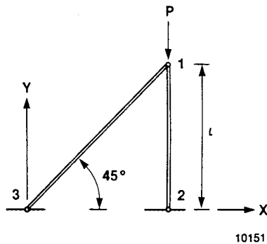
Figure 19. Truss structure.
