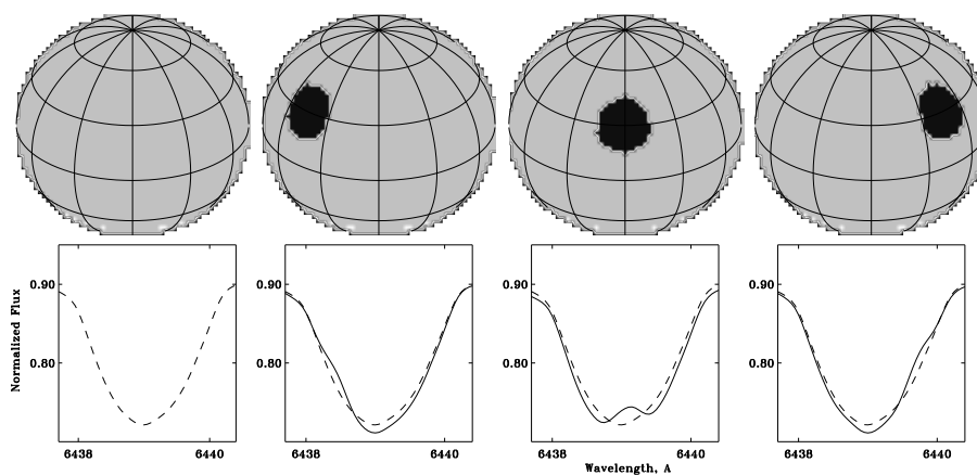
Figure 2: Spectral line profiles for a model fast rotating star with no spots (dashed line) and with a spot moving across the disk as the star rotates (solid line). See also animation at http://www.astro.phys.ethz.ch/staff/berdyugina/private/StellarActivity/StellarAct.html
