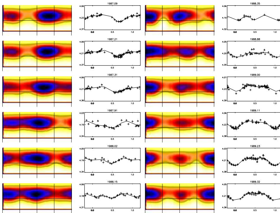
Figure 1: Light curve inversion results for the RS CVn star \sigma Gem (Berdyugina & Henry, in preparation). The first and third columns are maps of the spot filling factor. Darker regions indicate larger values. Observed and calculated V-band light curves are shown in the second and fourth columns by crosses and lines, respectively. The images also illustrate a flip-flop event that occurred in 1988: the active region near the phase 0.5 has diminished for about one year, while the region near the phase 0.0 has increased in size (see discussion of the flip-flop phenomenon in Section 6.2).
