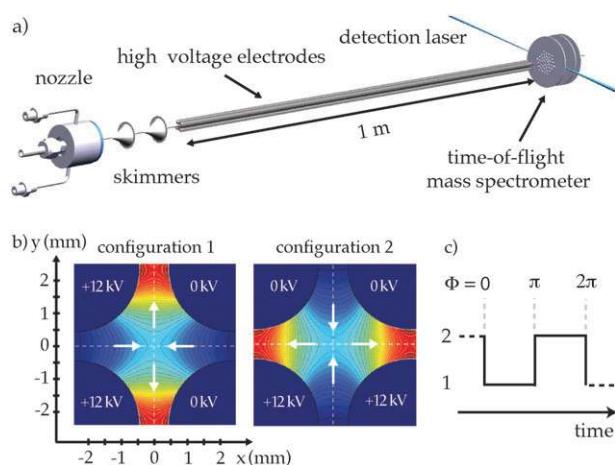
Fig. 4 (a) Scheme of the experimental setup used for alternating gradient focusing of high-field-seeking molecules. (c) Switching in a square wave pattern between the two electric field configurations shown in (b) results in a net focusing effect when the appropriate frequency is used.
