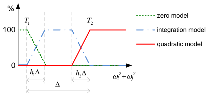
Figure 6. Defined probabilities of the interacted three models.
