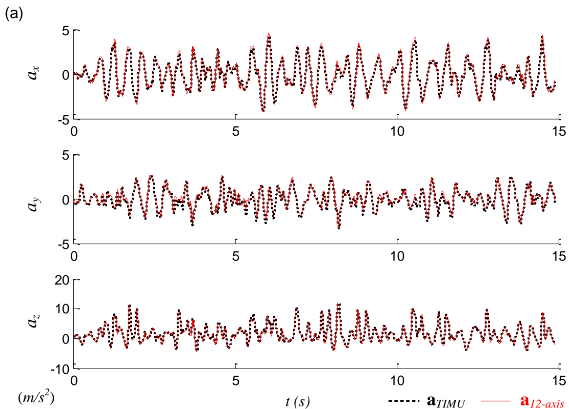
Figure 10. Comparison of states obtained from the traditional IMU (thick black dashed line) and the 12-axis IMU (thin red solid line): (a) linear acceleration, (b) angular acceleration, and (c) angular velocity.
