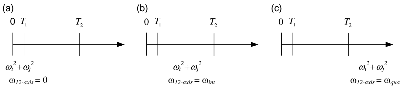
Figure 4. Three different computation methods categorized by the magnitude of the quadratic terms: (a) 0 \leq \omega_i^2 + \omega_j^2 \leq T_1 ; (b) T_1 \leq \omega_i^2 + \omega_j^2 \leq T_2 ; (c) \omega_i^2 + \omega_j^2 \geq T_2 .
