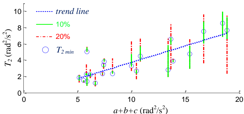
Figure 8. The relation between amplitude of motion and T_{2min} .
