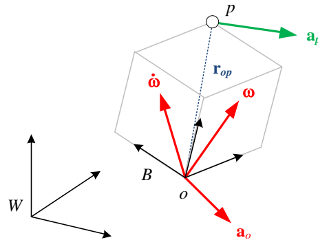
Figure 1. General description of the accelerated body in the inertial frame.
