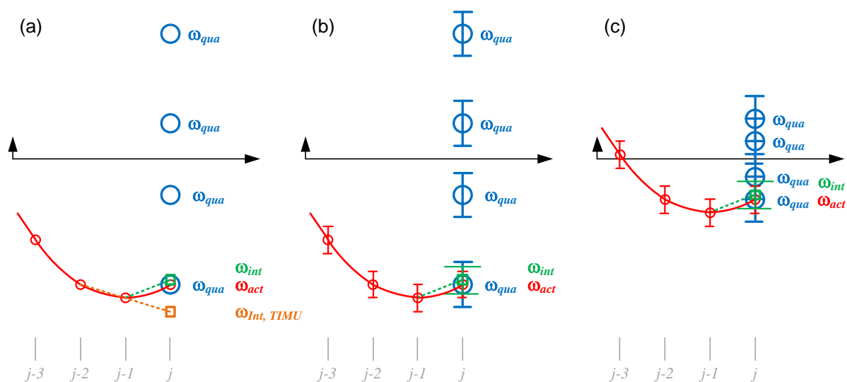
Figure 3. Various scenarios of selecting the correct angular velocity from the eight candidates deriving from the quadratic method: (a) “perfect world” with no estimate error, the true angular velocity (red line) is precisely sampled (red circle). The initial guess derived from integration method is represented in green color. (b) Normal situation where all computed data have certain variances (shown in error bar). (c) Normal situation when the magnitude of the angular velocity is small and the correct solution is hard to pick.
