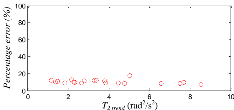
Figure 9. The relationship between T_2 and the ratio of RMSE and amplitude of angular velocity.
