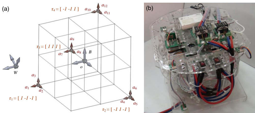
Figure 2. (a) The configuration of four 3-axis accelerometers that yields the best condition number for structure matrix \mathbf{S}(\mathbf{r}_m) . (b) The experimental apparatus.
