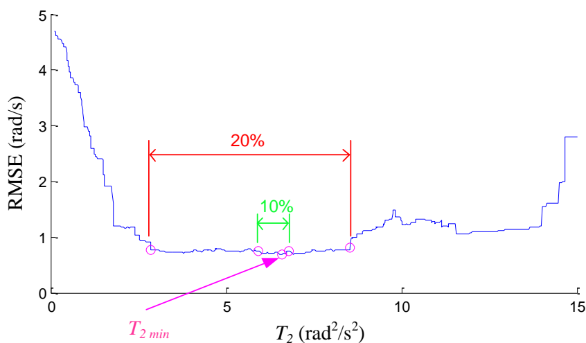
Figure 7. The relationship between T_2 and the RMSE between \omega_{TIMU} and \omega_{I2-Axis} .
