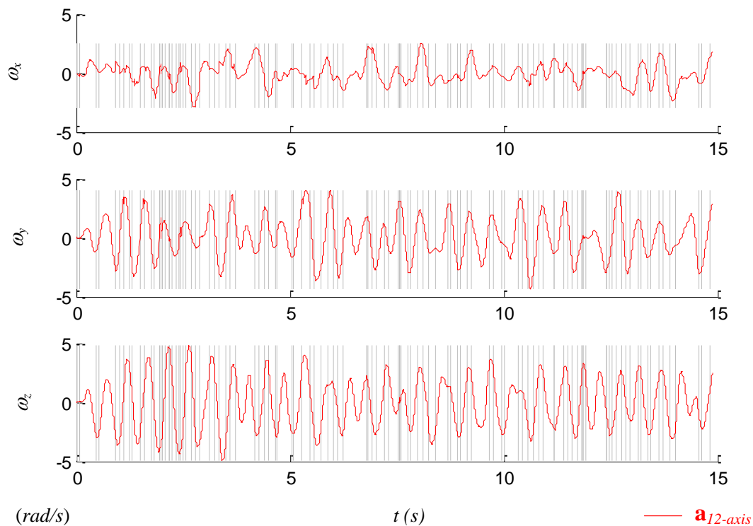
Figure 12. The timing of switching (grey lines) between the integration method and the quadratic methods.
