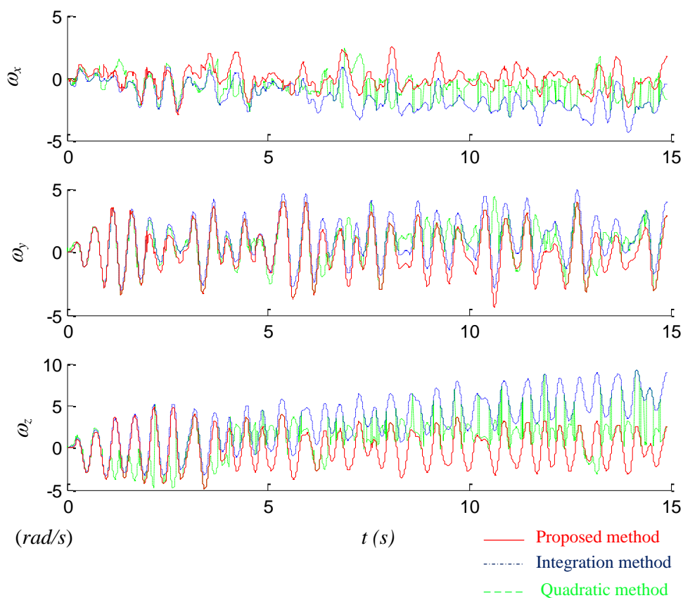
Figure 11. Comparison of the angular velocity derived from three different methods: integration method (blue dash-dotted line), quadratic method (green dashed line), and proposed method (red solid line).
