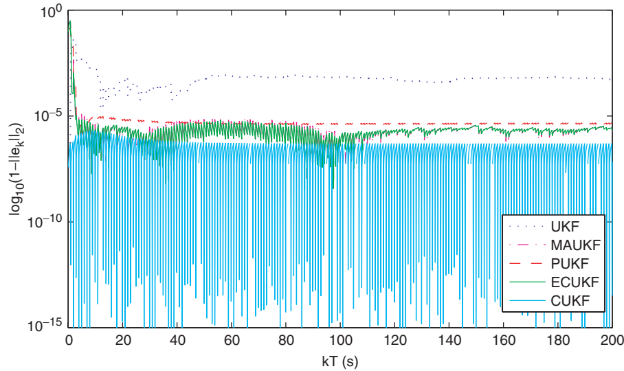
Figure 4. Estimation error of the quaternion vector norm using UKF ( \cdots ), ECUKF (thick \text{—} ), PUKF ( \text{---} ), MAUKF ( \text{-}\cdot\text{-} ) and CUKF (thin \text{—} ) algorithms. The ECUKF and MAUKF estimates almost coincide, while the constraint error for PUKF is slightly larger than the constraint error for ECUKF and MAUKF. CUKF estimates satisfy the equality constraint at machine precision at most times.
