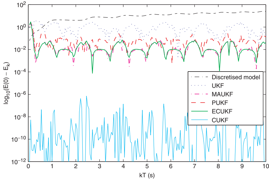
Figure 5. Estimation error of the total energy E(0) for the discretised pendulum (95)–(96) for UKF ( \cdots ), MAUKF (thick -\cdot-\cdot- ), PUKF ( --- ), ECUKF (thick — ) and CUKF (thin — ) with \sigma_v=0.25 . For comparison, the thin dot-dashed line, which is above the remaining lines, refers to the energy E_k calculated from data-free simulation of the discretised model (95). ECUKF and MAUKF estimates almost coincide, while CUKF estimates satisfy the equality constraint at machine precision at most times.
