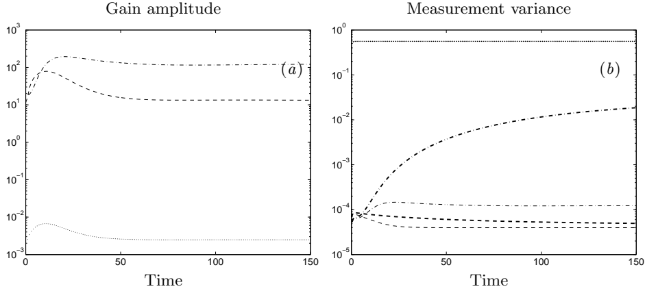
FIGURE 9. Time evolution of the peak absolute value of the gains and the variance of the measurements for the wavenumber pair \{0, 2\} . (a) Peak absolute value of the gains for the measurements of (dot-dashed) \tau_x , (dashed) \tau_z , and (dotted) wall pressure. (b) Variance of the measured signal (thick lines) and the measurement error (thin lines), with same line types as in part (a).
