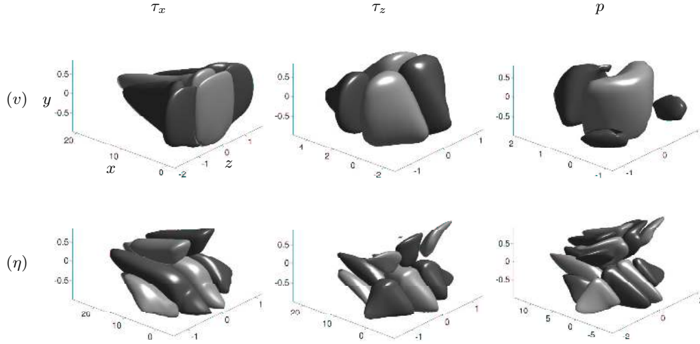
FIGURE 12. The steady-state convolution kernels relating the (left) \tau_x , (centre) \tau_z , and (right) p measurements at the point \{x = 0, y = -1, z = 0\} on the wall to the estimator forcing on the interior of the domain for the evolution equation for the estimate of (top) v and (bottom) \eta . Visualised are positive (dark) and negative (light) isosurfaces with isovalues of \pm 5\% of the maximum amplitude for each kernel illustrated.
