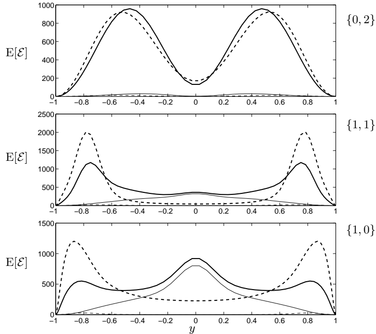
FIGURE 6. The distribution in y of the expected energy at statistical steady state of the flow (thick lines) and the estimation error (thin lines) for three wavenumber pairs: ( top ) \{0, 2\} , ( centre ) \{1, 1\} , and ( bottom ) \{1, 0\} , and for two different wall-normal distributions of the external perturbations: p = 0 (solid) and p = 5 (dashed).
