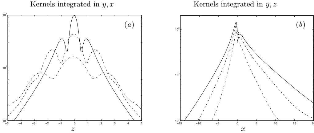
FIGURE 13. Decay of the pressure kernel forcing the streamwise velocity component of the state estimate, (a) integrated in the streamwise and wall normal direction for (solid) d_x = d_z = 0.2 , (dashed) 0.7, and (dot-dashed) 1.3, and (b) integrated in the spanwise and wall-normal directions for (solid) Re = 3000 , (dashed) 2000, (dot-dashed) 1000.
