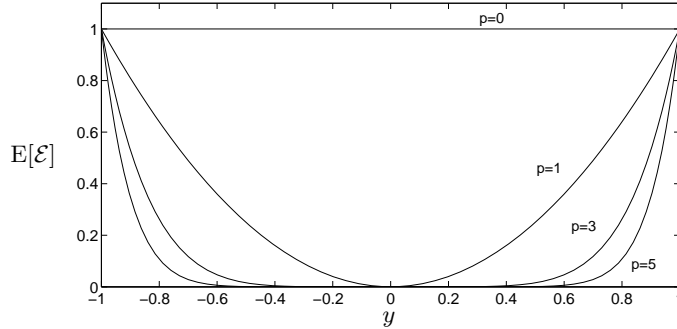
FIGURE 5. The wall-normal distribution of the variance in the augmented form of the external disturbance parameterization. Four cases are shown, corresponding to p = 0, 1, 3, 5 .
