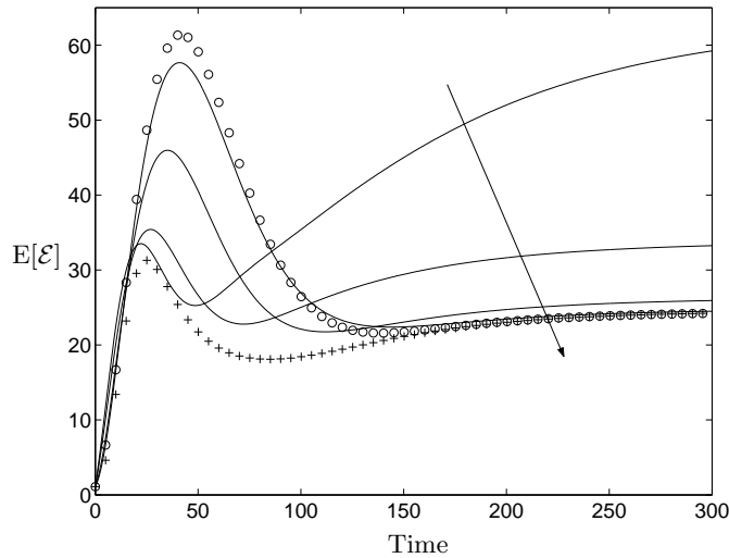
FIGURE 10. Energy of the expected estimation error for gains selected from the time-varying solution to the DRE and applied as constant-gain feedback, tested at the wavenumber pair \{0, 2\} . Gains are selected from times 20, 40, 60, and 80 (solid lines, with later times in the direction of the arrow), as compared with the (constant) solution of the ARE ( \circ ) and the full (time-varying) solution of the DRE ( + ).
