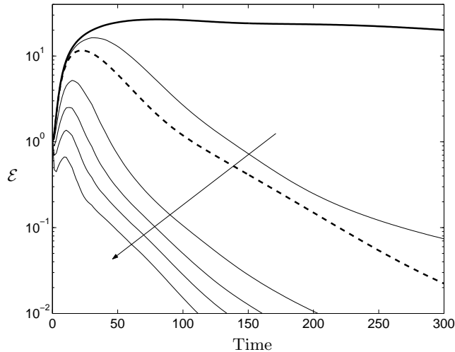
FIGURE 15. The time evolution of the energy of an infinitesimal localised flow perturbation (thick solid line) and the energy of the estimation error of the same flow using (dashed line) the steady state kernels determined from the solution of the ARE as well as (thin solid lines) a gain scheduled set of kernels computed using values of c_2 = 0.05, 0.1, 0.25, 0.5, and 1 , increasing in the direction of the arrow. Note that the energy \mathcal{E} has been normalized by energy of the initial flow perturbation.
