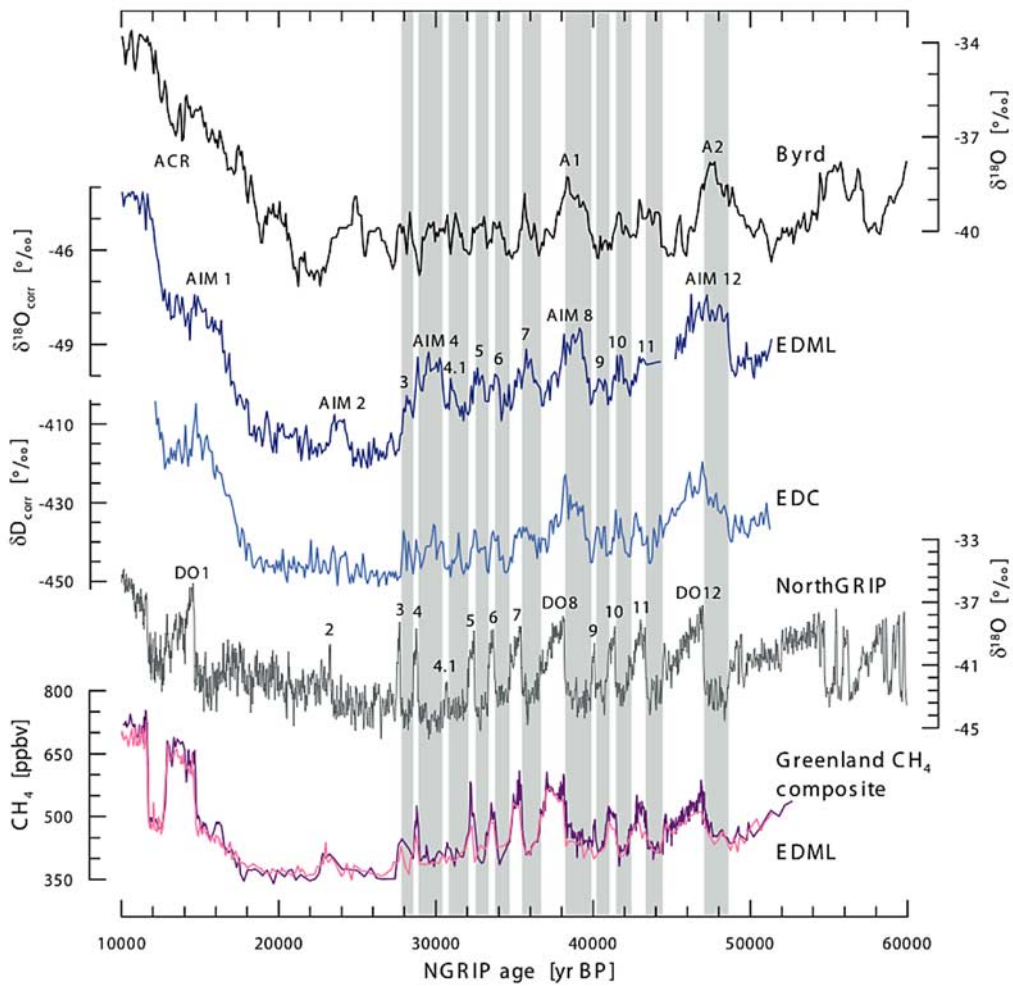
Figure 6. Methane (CH 4 ) synchronization of the ice core records of δ 18 O as a proxy for temperature reveals one-to-one association of Antarctic warming (Antarctic isotope maxima (AIM)) events with corresponding Greenland cold (stadial) events (Dansgaard/Oeschger (DO)) covering the period 10,000–60,000 years ago. EDML, EPICA core from Dronning Maud Land Antarctica; Byrd, core from West Antarctica; EDC, core from East Antarctica; NGRIP, core from north Greenland. Gray bars refer to Greenland stadial periods. Greenland CH 4 composite curve is blue; EDML CH 4 signal is pink. Figure modified from EPICA Community Members [2006] by H. Fischer.
