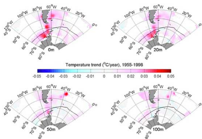
Figure 16. Trends in ocean summer temperature during 1955–1998, for four different depth levels (surface, 20 m, 50 m, and 100 m). Grid cells with no data are left white. Note the significant warming trend observed close to the western Antarctic Peninsula: this is strongly surface intensified, decaying virtually to zero at 100 m depth. From Meredith and King [2005, Figure 2].
