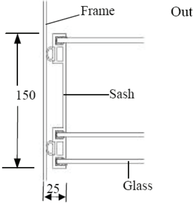
Figure 5. Frame profile made from fiber glass reinforced polyester with three layers of glass (Lautsen and Svendsen, 2005). The frame U-value is 1.33 W/m 2 K.
