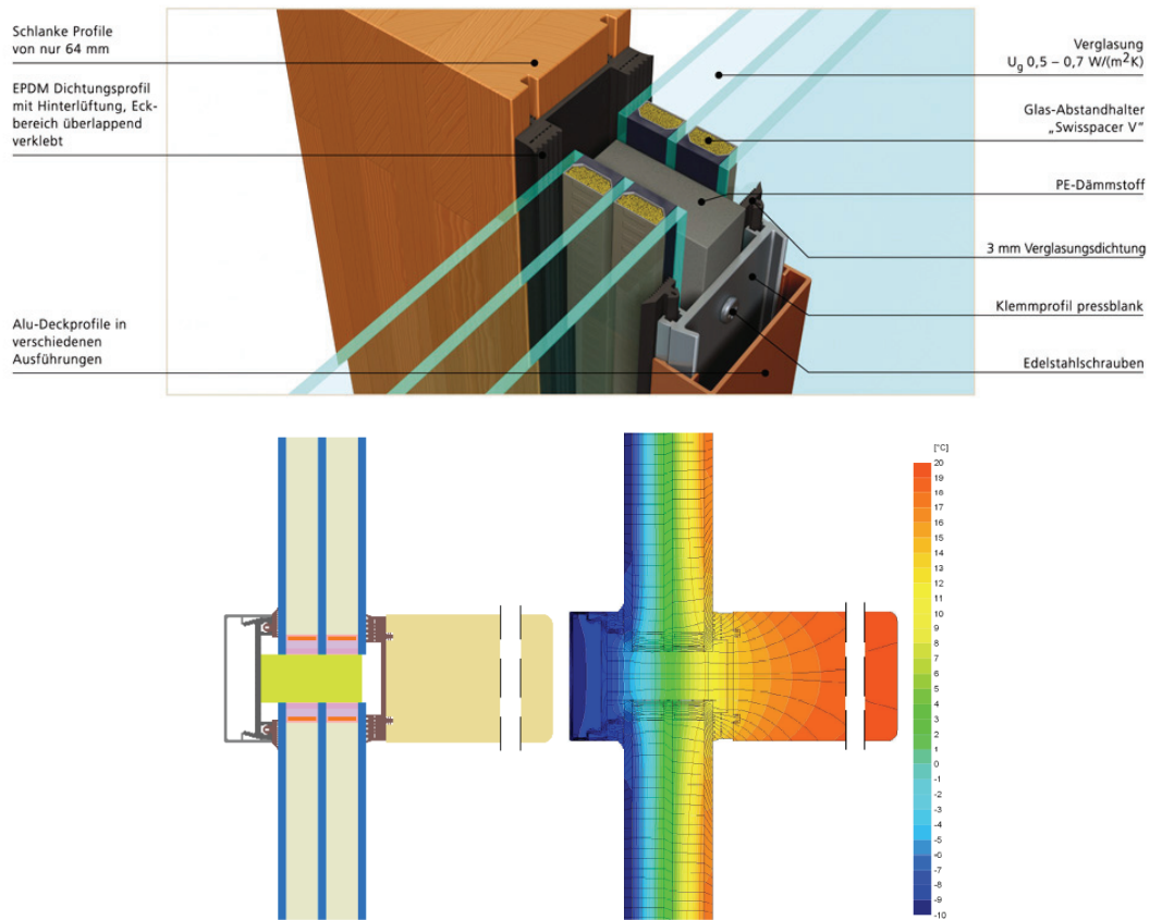
Figure 28. Example of a glass facade system with low U-value - ON TOP PLUS by Endl-Wagner GmbH. Picture on the top, one schematic drawing to the left and one temperature profile to the right. Wood-Al profile. Frame U-value U_f = 0.65 \text{ W/m}^2\text{K} . From http://www.passiv.de and www.endl.at .
