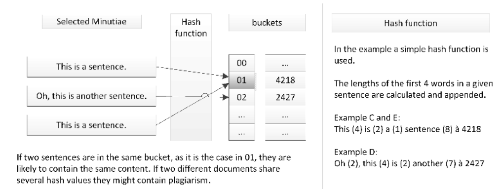
Figure 3: Concept of fingerprinting
