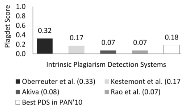
Figure 6: Plagdet scores for intrinsic PDS in PAN-PC'11 Source: (Potthast, Eiselt, et al., 2011)
