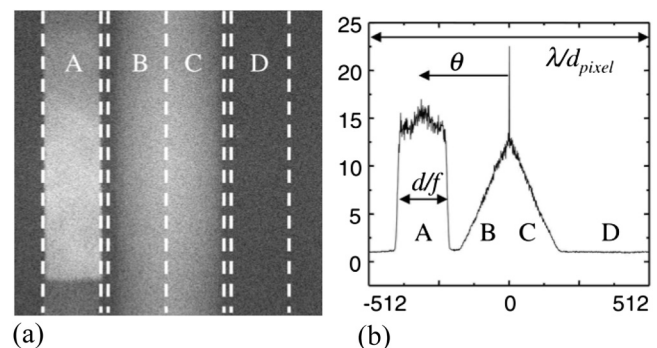
Fig. 5 k -space image (a) and column average of this image (b) with the regions: signal (A), decorrelation noise (B and C), and shot noise (D). 46
