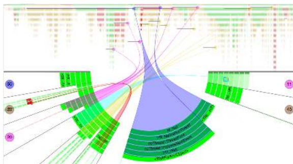
Figure 10: SyncTrace [KTD13] visualization shows thread call stacks and relationships between them. Image courtesy of B. Karran.
