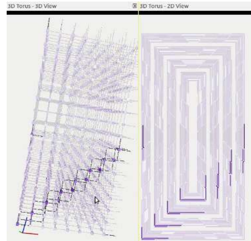
Figure 2: A screenshot of Boxfish [LLB*12,ILG*12] showing a selected set of nodes in a 3-dimensional torus network. Nodes are arranged in a 3-dimensional graph with links denoted by edges (left) and an orthogonal projection shows a subset of the edges without occlusion (right).
