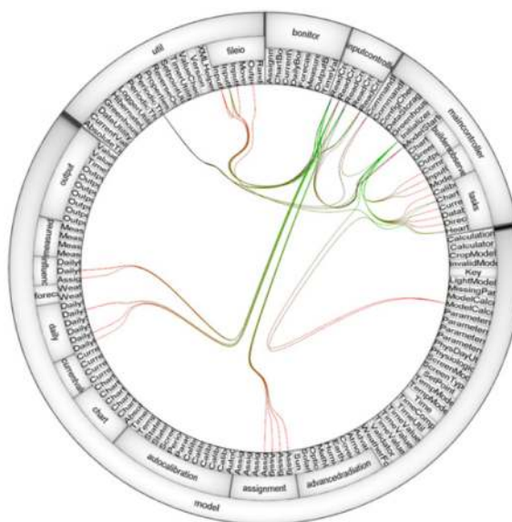
Figure 6: Inner nodes represent different methods. Edges show caller-callee relationships. The edge color gradient can be used to denote the call direction or to show the call time-less recent (light) to most recent (dark). Radial icicle plots show the software structure, which provides insight into how different packages are linked to each other. Image ©2007 IEEE. Reprinted, with permission, from [CHZ*07].
