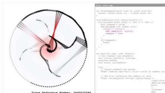
Figure 5: Memory hierarchy visualization by [CR11]. Left: Addresses are represented as points, and different sets of points represent different memory resources. The outer ring represents main memory, the outer four arcs of points represent L2 cache, and the inner two arcs represent L1 cache. Lines between points denote migration of data between resources. Right: Simulated transactions are associated with the lines of code which caused them. Image courtesy of P. Rosen.
