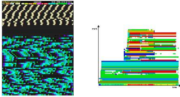
Figure 3: Left: Memory visualization by [GT89]. Memory address space depicted as a 1-dimensional array wrapping down several rows. Blocks indicate allocations along address space, color legend indicates variable data types. Printed with author’s permission. Right: Memory visualization by [MT07]. Allocations depicted as 2D blocks with address space on the vertical axis and time on the horizontal axis. Image courtesy of A. Telea.
