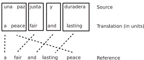
Fig. 1 Source, translation (in units) and reference example. Translation and reference differ in word order.
