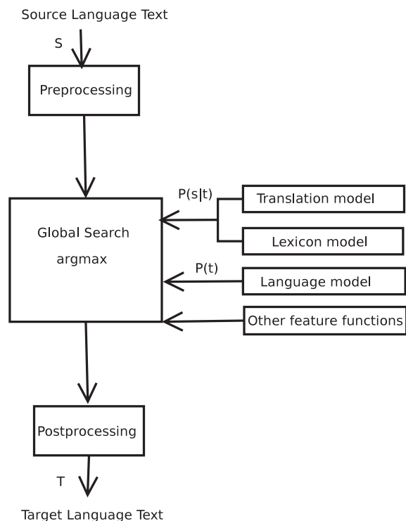
Fig. 2 Architecture of the SMT translation approach based on the log-linear framework approximation: different feature functions are combined in the global search.
