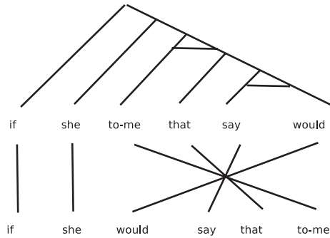
Fig. 4 Example of reordering using ITG. The alignments are added below the tree, and the horizontal bars in the tree indicate the swap.
