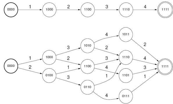
Fig. 3 Permutation graph: monotonic (top) and reordered using IBM constraints (bottom) search.
