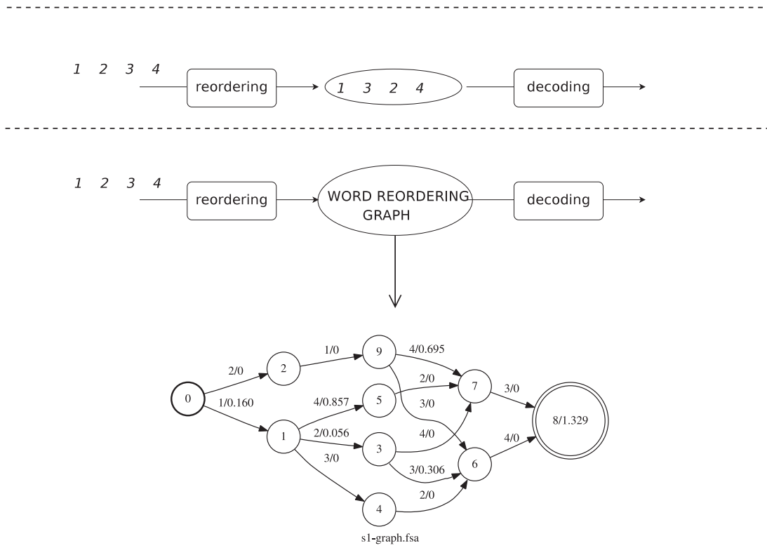
Fig. 5 Source reordering approaches: deterministic reordering (up) and input reordering graph (down).
