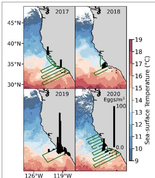
FIGURE 11 | Densities of anchovy eggs (black bars) captured in the Continuous Underway Fish Egg Sampler during winter CalCOFI cruises, 2017–2020. Green lines indicate the ship's positions during sampling. Data were overlaid on satellite-derived sea surface temperatures (AVHRR 1.4-km resolution).
