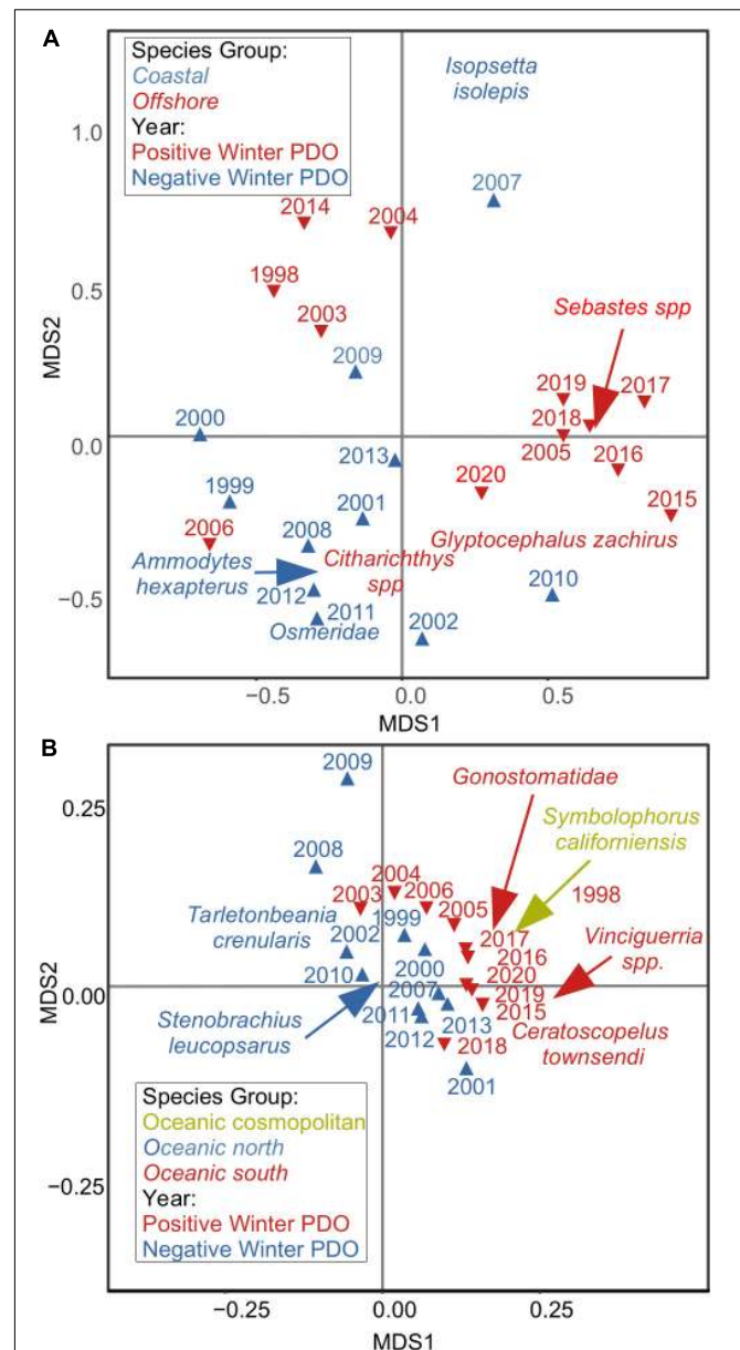
FIGURE 10 | Non-metric multidimensional scaling of ichthyoplankton species by year for winter cruises at the Newport Hydrographic Line (A) and on CalCOFI lines 80 and 90 (B). Symbol colors indicate positive/negative PDO, and species colors indicate their preferred distributions. Arrows denote actual species positions where they have been moved to improve clarity.
