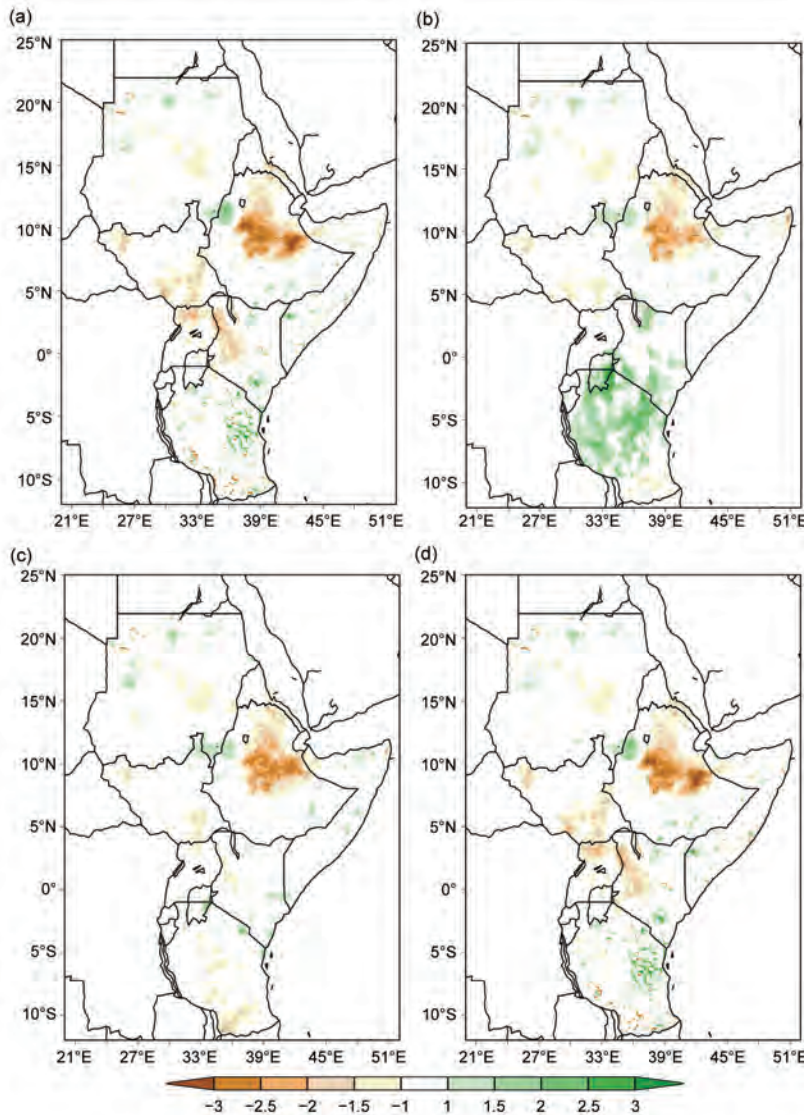
FIG. 7.20. SPI indices for eastern Africa for Oct 2014–September 2015 at (a) 3-month, (b) 6-month, (c) 9-month, and (d) 12-month times scales, based on 1981–2015 rainfall climatology.
