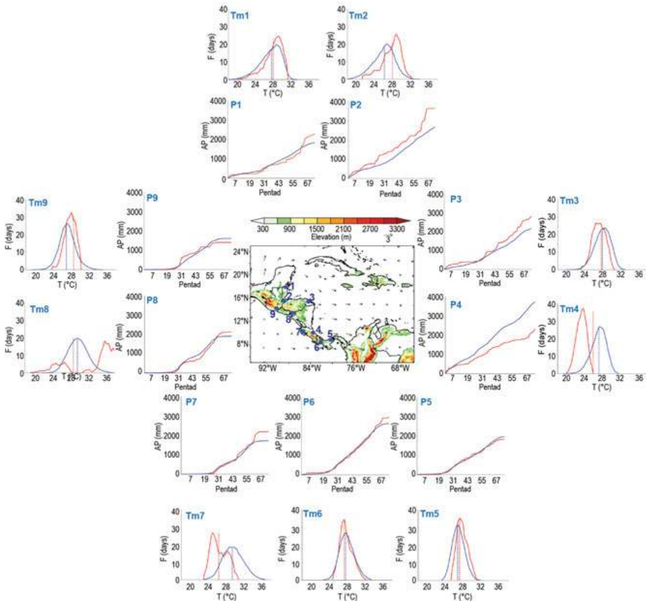
Fig. 7.8. Mean surface temperature ( T_m ; °C) frequency ( F ; days), and accumulated pentad precipitation ( P ; mm) time series are shown for nine stations (blue dots) in Central America: (1) Philip Goldson International Airport, Belize; (2) Puerto Barrios, Guatemala; (3) Puerto Lempira, Honduras; (4) Puerto Limón, Costa Rica; (5) Tocumen International Airport, Panamá; (6) David, Panamá; (7) Liberia, Costa Rica; (8) Choluteca, Honduras; and (9) Puerto San José, Guatemala. The blue solid line represents the 1981–2010 average values and the red solid line shows 2020 values. Vertical dashed lines show the mean temperature for 2020 (red) and the 1981–2010 period (blue). Vectors indicate July wind anomalies at 925 hPa (1981–2010 base period). Shading depicts regional elevation (m). (Sources: NOAA/NCEI and CA-NWS.)
