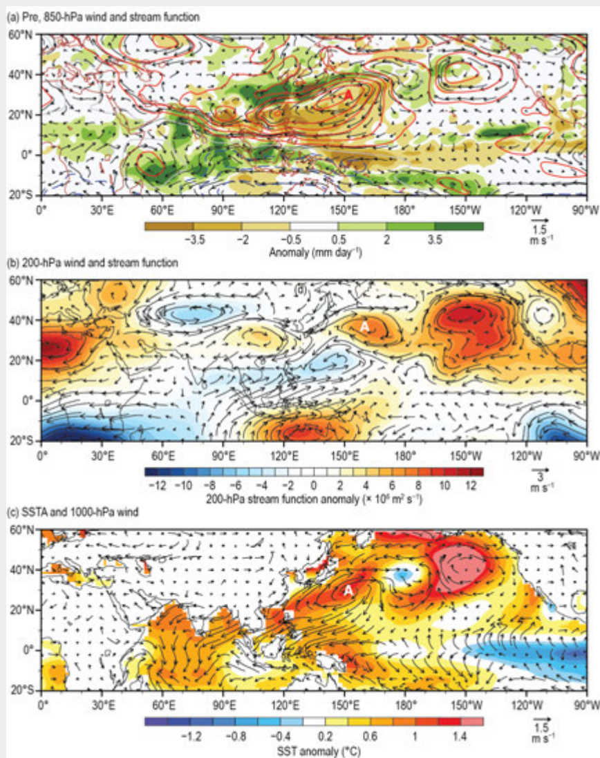
Fig. SB7.3. The horizontal patterns of (a) anomalous precipitation (shading, \text{mm day}^{-1} ) and wind (vector, \text{ms}^{-1} ) and stream function (contour 10^6 \text{ m}^2 \text{ s}^{-1} ) anomalies at 850 hPa, (b) anomalous wind (vector, \text{ms}^{-1} ) and stream function (contour 10^6 \text{ m}^2 \text{ s}^{-1} ) at 200 hPa, and (c) anomalous SST (shading, ^{\circ}\text{C} ) and wind at 1000 hPa (vector, \text{ms}^{-1} ) averaged in Jun–Jul (JJ) 2020. The baseline for the mean climatology is 1979–2020. Letter “A” denotes the anomalous anticyclonic center in the WNP.
