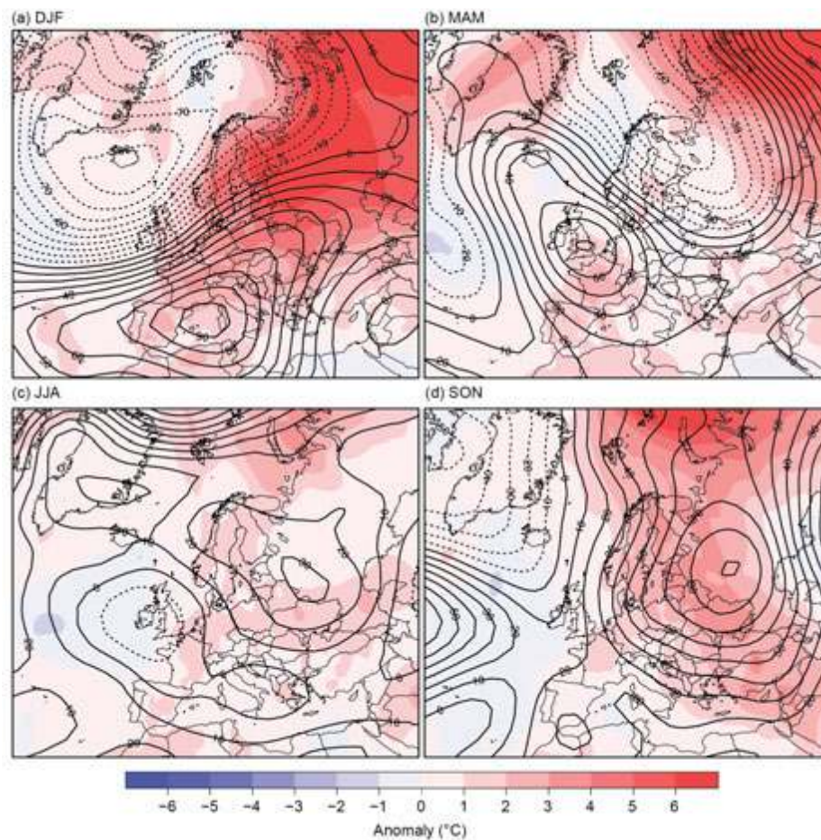
Fig. 7.39. Seasonal anomalies (1981–2010 base period) of 500-hPa geopotential height (contour; m) and surface air temperature (shading; °C) using data from the NCEP/NCAR reanalysis and DWD, respectively, for (a) DJF 2019/20, (b) MAM 2020, (c) JJA 2020, and (d) SON 2020.
