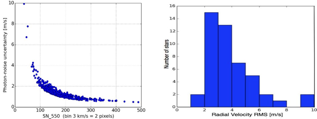
Figure 7. Theoretical uncertainty based on SNR and radial velocity scatter for the SOPHIE spectrograph. (Courtesy of Francois Bouchy)
