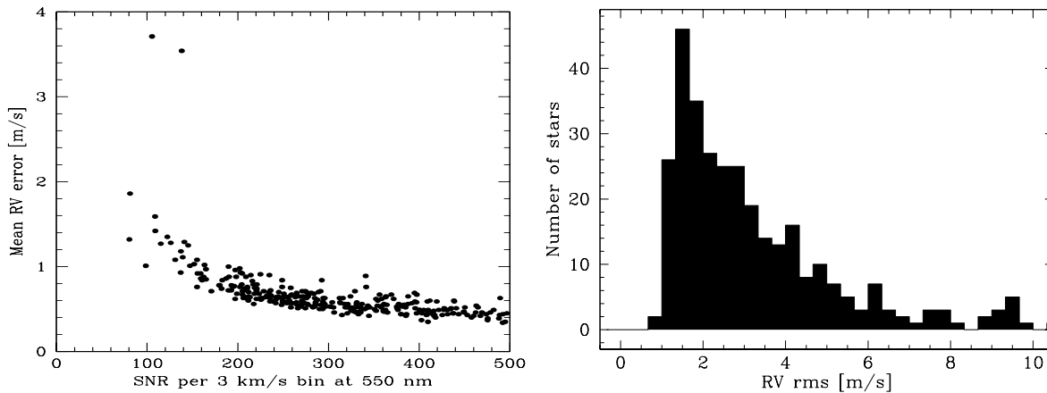
Figure 6. Single measurement precision as a function of SNR (left) and radial velocity scatter (right) at HARPS for the target sample of FGK dwarfs to search for super Earth and Neptune mass exoplanets with HARPS. (Courtesy of Christophe Lovis)
