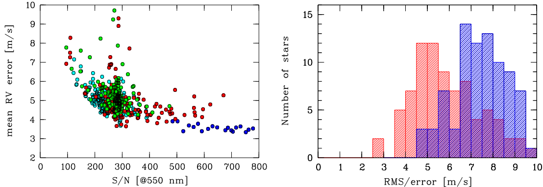
Figure 3. (left) Estimated single measurement precision as a function of SNR using the Tull spectrograph on the 2.7-m Harlan Smith Telescope at McDonald Observatory. Different color plot symbols are for different stars. (right) Radial velocity scatter (right) for the stars observed with this same spectrograph at McDonald Observatory. (Courtesy of Michael Endl)
