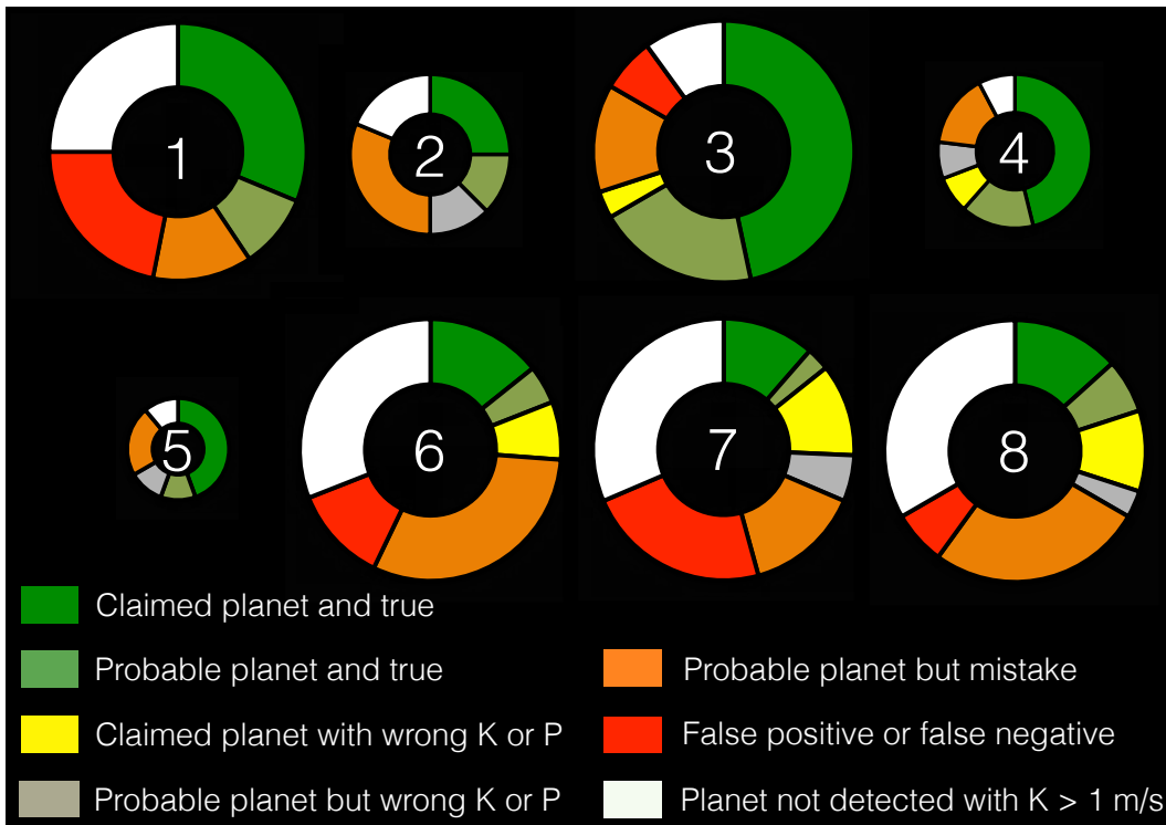
Figure 20. Summary of the result of the RV fitting challenge for teams 1 to 8. The size of the circles represents the number of systems analyzed: 14 systems for the large size circle, 5 for the medium size and 2 for the smallest size. The meaning of the colors are defined in the legend and in the text (Courtesy of Xavier Dumusque)
