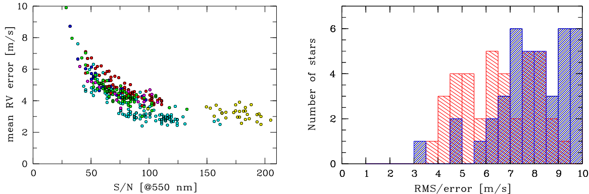
Figure 5. Radial velocity precision as a function of SNR (left) and radial velocity scatter (right) for HRS. (Courtesy of Michael Endl)
