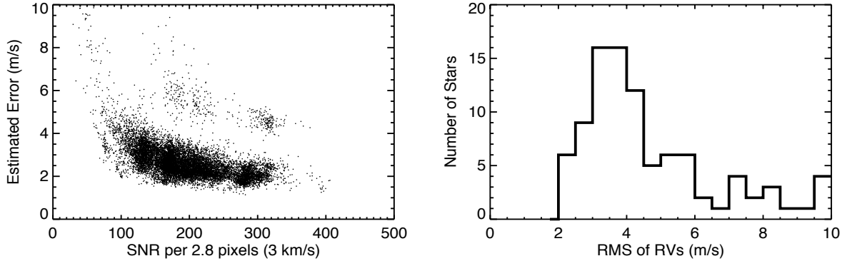
Figure 12. Estimated precision (left) and radial velocity scatter (right) for Doppler measurements obtained by the California Planet Search team using the Levy Spectrograph at the Automated Planet Finder. (Courtesy of Andrew Howard)
