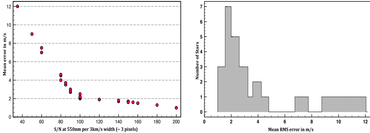
Figure 10. Precision and radial velocity scatter for PARAS. (Courtesy of Abhijit Chakraborty) The plot on the left shows the nightly RV scatter as a function of SNR in 3 \text{ km s}^{-1} bins and the plot on the right is a histogram of the long term rms scatter for 27 bright stars.
