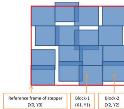
Figure 15. Example of the pixel image blocks required to create a 2k x 2k pixel CCD with exaggerated random position errors relative to the reference frame (image credit to e2V technologies).
