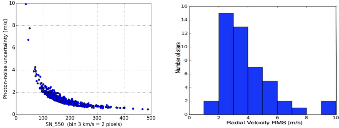
Figure 7. Theoretical uncertainty based on SNR and radial velocity scatter for the SOPHIE spectrograph. (Courtesy of Francois Bouchy)
