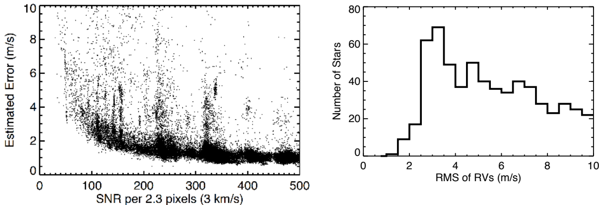
Figure 2. Radial velocity precision (left) and rms velocity scatter for Doppler measurements by the California Planet Search team using the HIRES at Keck. (Courtesy of Andrew Howard)
