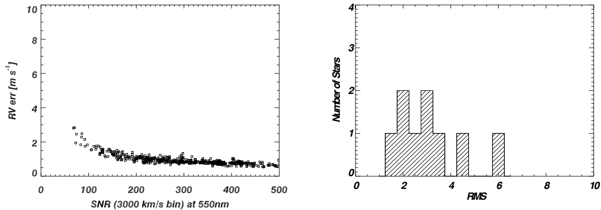
Figure 9. Single measurement precision (left) and radial velocity scatter for ten bright stars observed with CHIRON at CTIO. (Courtesy of Debra Fischer)
