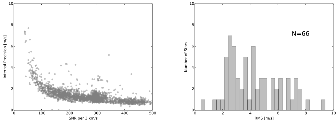
Figure 13. Radial velocity precision as a function of SNR (left) and velocity rms (right) for the Lick Planet Search team with the Levy Spectrograph at the Automated Planet Finder. (Courtesy of Greg Laughlin)
