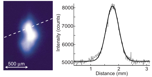
FIG. 12. (Color online) Blue fluorescence image (false color) of the uncompressed MOT for 780 nm excitation and 776 nm probe. 1 s exposure with 21 G/cm magnetic field gradient, 85 °C vapor cell filter temperature. The fluorescence intensity is shown for a profile along the dashed line, with a Gaussian fit.
