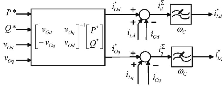
Figure 3: Power controller [22]
