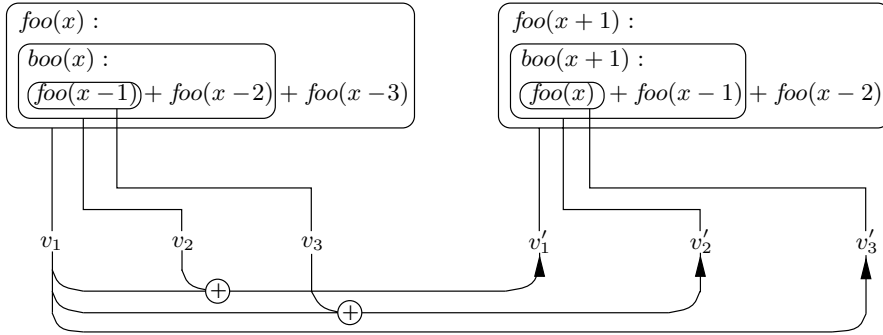
Fig. 6. Transitive dependencies.
