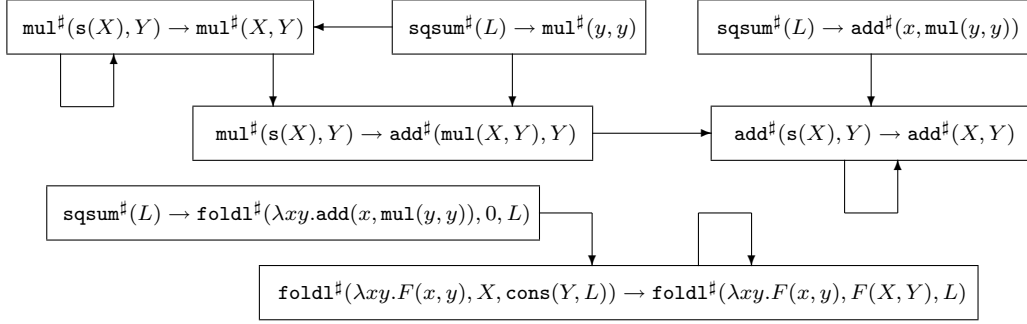
Figure 1: static dependency graph of R_{\text{sqsum}}
