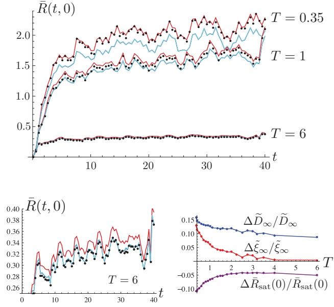
FIG. 13. (Color online) Top: Time evolution of the maximum of the correlator peak \bar{R}(t,0) at fixed temperature T \in \{0.35, 1, 6\} measured numerically (black dots) or predicted by the fitting functions via \bar{R}^{\text{fit}}(t,0) = \mathcal{R}_{\xi=1}^{\text{fit}}(0) \tilde{D}_t^{\text{fit}} / \xi_t^{\text{fit}} (top) red for Gauss (35) and blue for SincG (36); (bottom) cyan for CubicS [(A2) and (A3)]. The curves for SincG and CubicS systematically coincide. Bottom left: Close-up of the high- T case, where the SincG and CubicS predict more accurately the peak at high T , whereas at low T Gauss seems more suited. Bottom right: Decrease in the relative differences between the Gauss and SincG parameters with increasing temperature, averaged on the large-time window t \in [25, 40] : \frac{\Delta \tilde{D}_\infty}{\tilde{D}_\infty} = \frac{\tilde{D}_\infty^{\text{SincG}} - \tilde{D}_\infty^{\text{Gauss}}}{\tilde{D}_\infty^{\text{SincG}}} , \frac{\Delta \tilde{\xi}_\infty}{\tilde{\xi}_\infty} = \frac{\tilde{\xi}_\infty^{\text{SincG}} - \tilde{\xi}_\infty^{\text{Gauss}} \xi_{\text{SincG}} / \xi_{\text{Gauss}}}{\tilde{\xi}_\infty^{\text{SincG}}} (see the end of Appendix A), and \frac{\Delta \bar{R}_{\text{sat}}(0)}{\bar{R}_{\text{sat}}(0)} = \frac{\bar{R}_{\text{sat}}^{\text{SincG}}(0) - \bar{R}_{\text{sat}}^{\text{Gauss}}(0)}{\bar{R}_{\text{sat}}^{\text{SincG}}(0)} .
