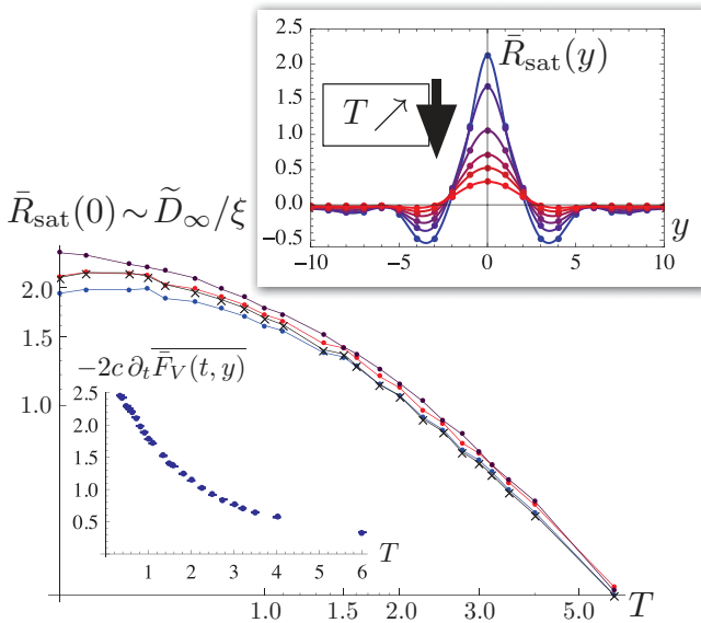
FIG. 6. (Color online) Temperature dependence of the maximum of \bar{R}_{\text{sat}}(y) over times t \in [25, 40] , measured by three different ways (from bottom to top): first, deduced by the SincG and Gauss fits as in Fig. 13 (respectively, blue and red dots); second, measured numerically directly \bar{R}_{\text{sat}}(0) (black crosses); and, third, measured indirectly from the linear slope of -2c \overline{\partial_t \bar{F}_V(t, y)} in Fig. 16 (purple dots) and systematically slightly overestimated. Upper inset: Saturation correlator \bar{R}_{\text{sat}}(y) for temperatures T \in \{0.35, 1, 2, 3, 4, 6\} (as indicated by the arrow) and t_{\text{min}} = 25 as listed in Appendix B. Lower inset: The excellent linear behavior of \overline{\partial_t \bar{F}_V(t, y)} yields vanishing error bars for the slope on the range t \in [25, 40] .
