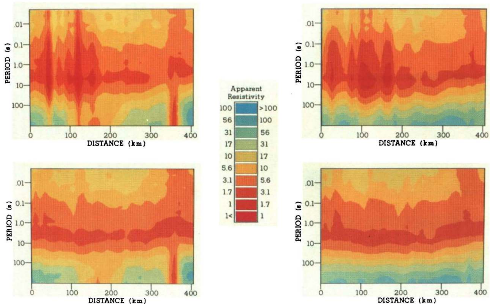
FIG. 15. (a) (top left) The uncorrected apparent resistivities observed in the E -polarization mode of induction plotted as contoured pseudosections. (b) (top right) The uncorrected apparent resistivities observed in the B -polarization mode of induction plotted as contoured pseudosections. (c) (bottom left) The corrected apparent resistivities observed in the E -polarization mode of induction plotted as contoured pseudosections. (d) (bottom right) The corrected apparent resistivities observed in the B -polarization mode of induction plotted as contoured pseudosections.
