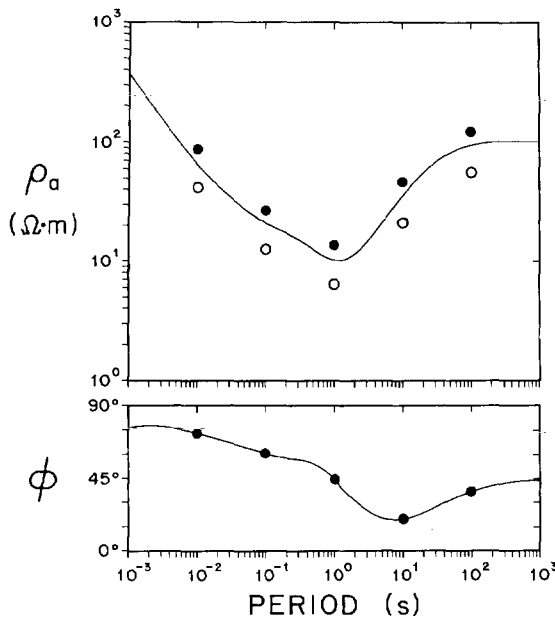
FIG. 3. One-dimensional modeling ( solid lines ) compared to voltage difference modeling (with 25 m electrode separation) of the structure shown in Figure 1 in the B -polarization mode of induction at locations of -70 m ( solid circles ) and -50 m ( open circles ), i.e., electrodes at distances of (-82.5, 57.5) and (-62.5, 37.5) , respectively, for the voltage difference modeling.
