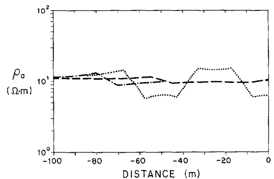
FIG. 4. Effect on the apparent resistivity of varying the electrode line length for the model shown in Figure 1 at a period of 1 s for electrode dipole separations of 25 m ( dotted line ), 50 m ( dashed-dotted line ), and 100 m ( dashed line ).
