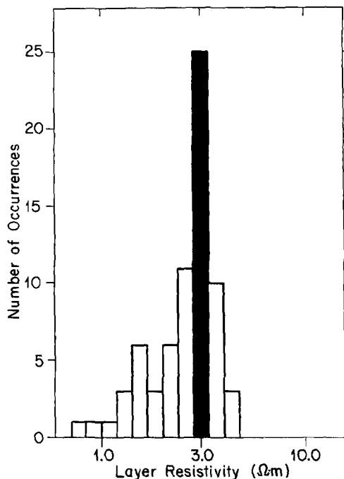
FIG. 14. Histogram of the 70 estimates of \rho_2 .
