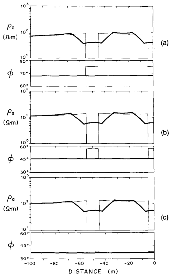
FIG. 2. Conventional point electric field modeling ( fine lines) compared to voltage difference modeling ( heavy lines), with an electrode line length of 25 m, for the structure shown in Figure 1 in the B -polarization mode of induction at (a) 0.01 s, (b) 1 s, and (c) 100 s periodicity. For the voltage difference modeling, the electrodes are positioned equidistantly about the given distance.
