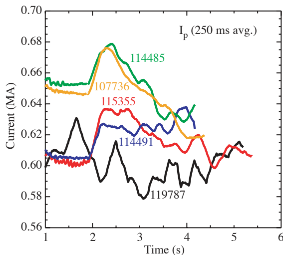
Fig.11. Plasma current vs. time for five different discharges. The indication is that, until the heating power pulse ends, these are all trending toward roughly the same level.
