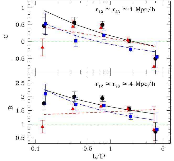
Figure 8. Deviations of Q_3 from the \Lambda CDM prediction as quantified by B and C (see equation 6; recall that, for the dark matter, B = 1 and C = 0 , as shown by the horizontal dotted line in each panel). Results are shown for all configurations of triangles with r_{12} \approx r_{23} \approx 4 h^{-1} \text{ Mpc} , as a function of luminosity. Circles, triangles and squares with error bars correspond to all, red and blue galaxies, respectively. Continuous, short-dashed and long-dashed lines show the corresponding predictions for all, red and blue galaxies using the best-fitting parameters listed in Table 3 and equation (9).
