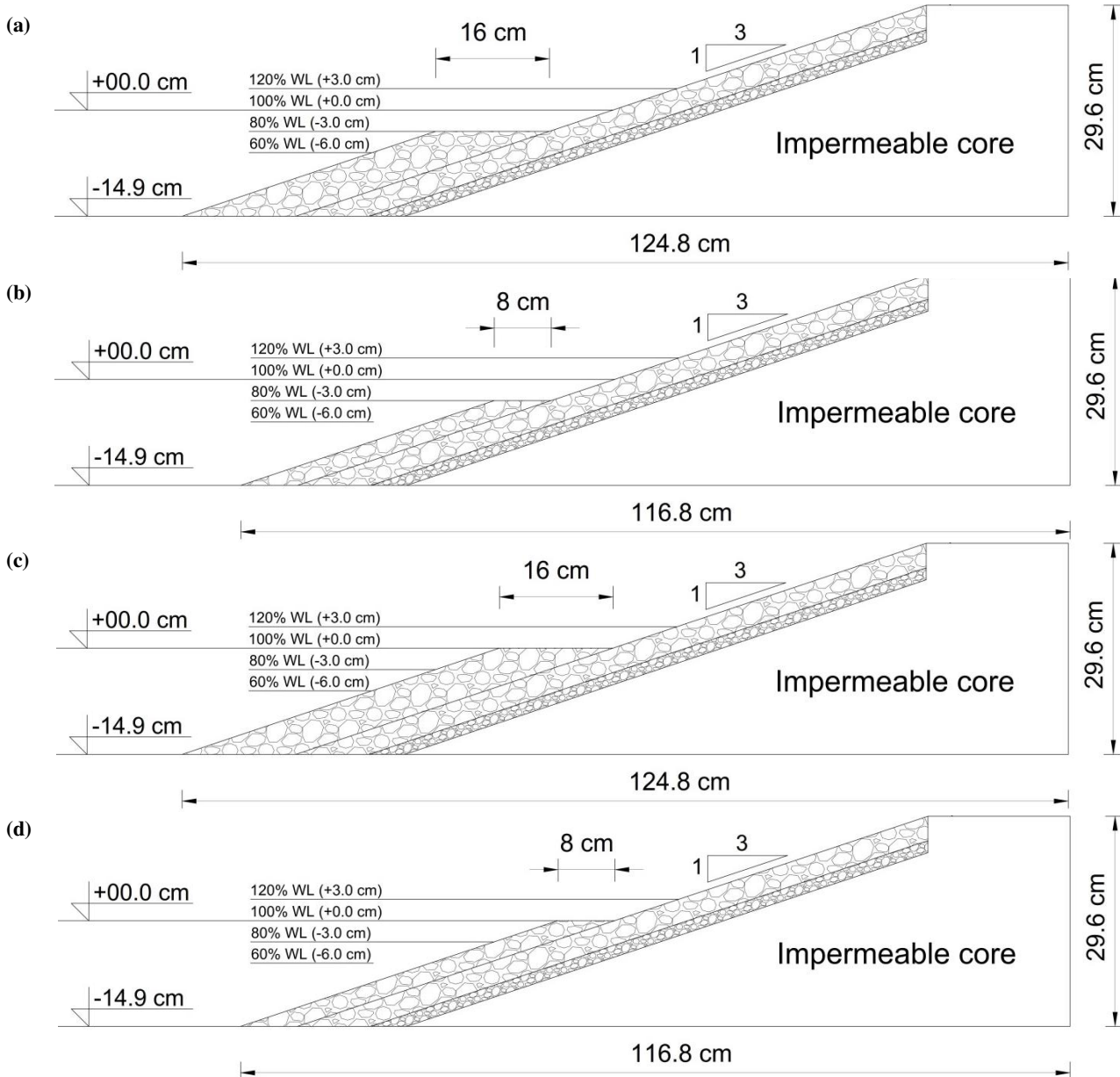
Figure 3. Structure geometries with berms (a: Wide berm at a level of "80% of the 100% WL"; b: Narrow berm at "80% of the 100% WL"; c: Wide berm at a level of the "100% WL"; d: Narrow berm at the "100% WL").
