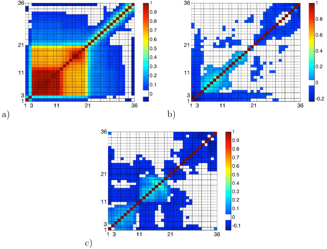
Figure 5: Matrices \Sigma_{ij}^C (panel a) , \Sigma_{ij}^F (panel b), and \Sigma_{ij}^B (panel c) describing the correlation between the time-step estimates of the i^{th} and j^{th} FTCLE, FTFLE, and FTBLE, respectively. See text. Parameters' value: C_o = 350 \text{ W m}^{-2} and d = 1 \times 10^{-8} \text{ s}^{-1} .
