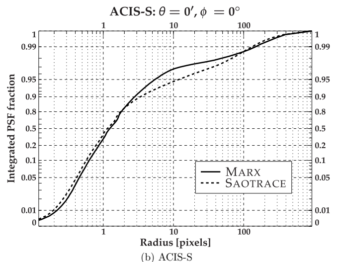
Figure 53. Encircled energy as a function of radius for an on-axis source on the ACIS-I and ACIS-S arrays. The source spectrum was assumed to be an absorbed power law with an absorbing column of 10^{21} cm ^{-2} and index of 1.7.
