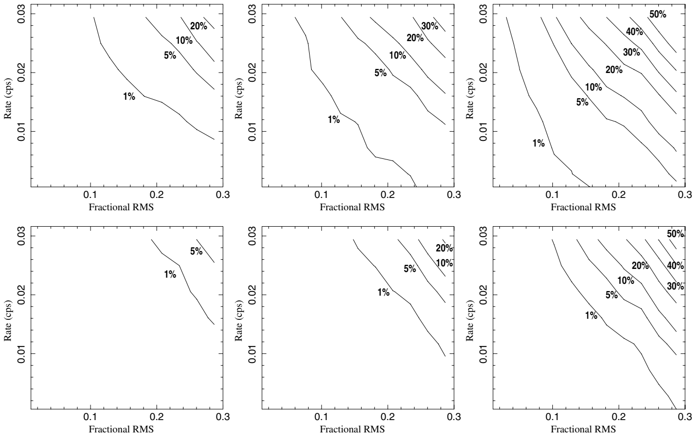
Figure 46. Contours for the fraction of simulated red noise light curves (as a function of simulated fractional rms and mean count rate) detected as variable with O \equiv \log_{10}(P^{-1}) > 2 (i.e., significantly variable at >99\% confidence). The top row corresponds to the results of the Kuiper test, whereas the bottom row corresponds to the Gregory–Loredo test. From left to right, the durations of the light curves were 20 ks, 50 ks, and 160 ks.
