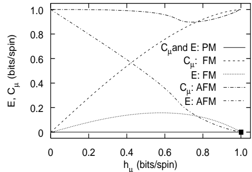
FIG. 2. The complexity-entropy diagram for a ferromagnet (FM), an anti-ferromagnet (AFM) and a paramagnet (PM): C_\mu and E plotted parametrically against h_\mu . For a given J , B was held constant— B = 0.30 (FM) and B = 1.8 (AFM)—as T was varied. All systems have C_\mu = 0 when h_\mu = 1 ; this is denoted by the square token.
